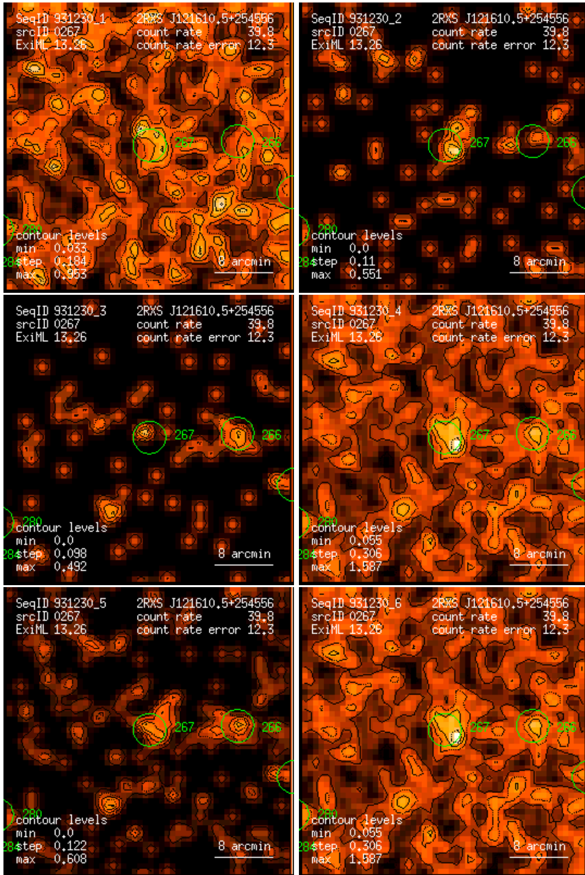
Figure 267: RASS 931230: detection 0267: band rate images, Gaussian filter: (1) PSPC channels 11 – 41, (2) 52 – 90, (3) 91 – 201, (4) 11 – 235, (5) 52 – 201, (6) 11 – 201. Broad band rates in counts/ks. Band rate contour levels in counts/ks/arcmin 2 .
