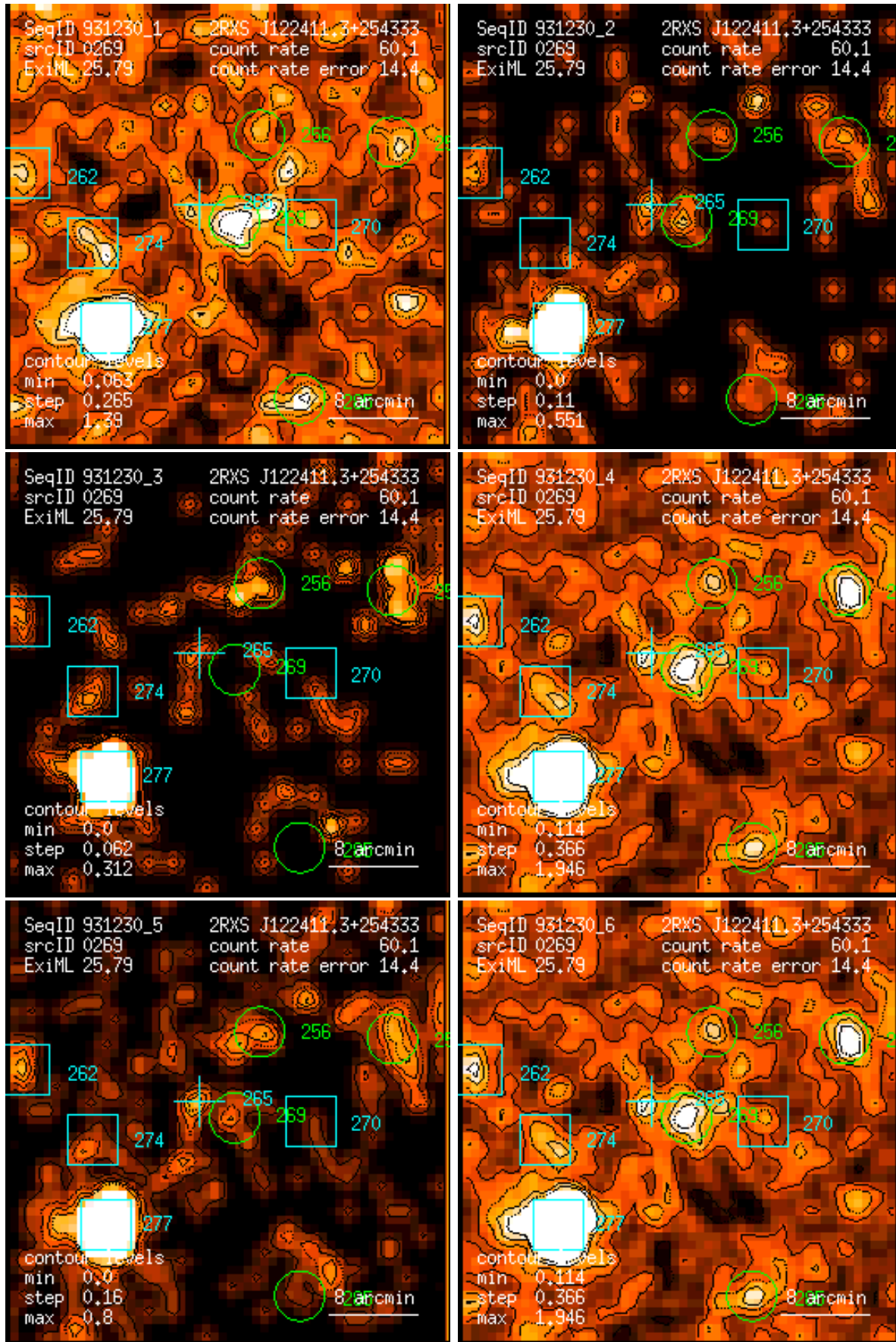
Figure 269: RASS 931230: detection 0269: band rate images, Gaussian filter: (1) PSPC channels 11 – 41, (2) 52 – 90, (3) 91 – 201, (4) 11 – 235, (5) 52 – 201, (6) 11 – 201. Broad band rates in counts/ks. Band rate contour levels in counts/ks/arcmin 2 .
