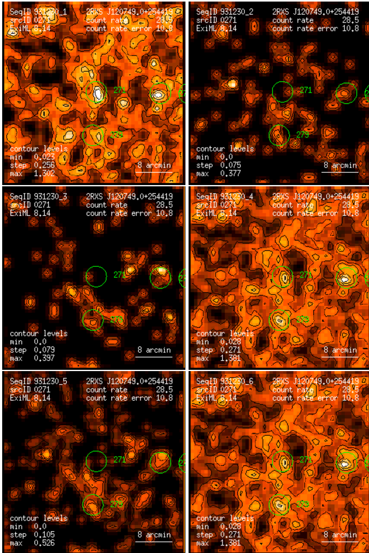
Figure 271: RASS 931230: detection 0271: band rate images, Gaussian filter: (1) PSPC channels 11 – 41, (2) 52 – 90, (3) 91 – 201, (4) 11 – 235, (5) 52 – 201, (6) 11 – 201. Broad band rates in counts/ks. Band rate contour levels in counts/ks/arcmin 2 .
