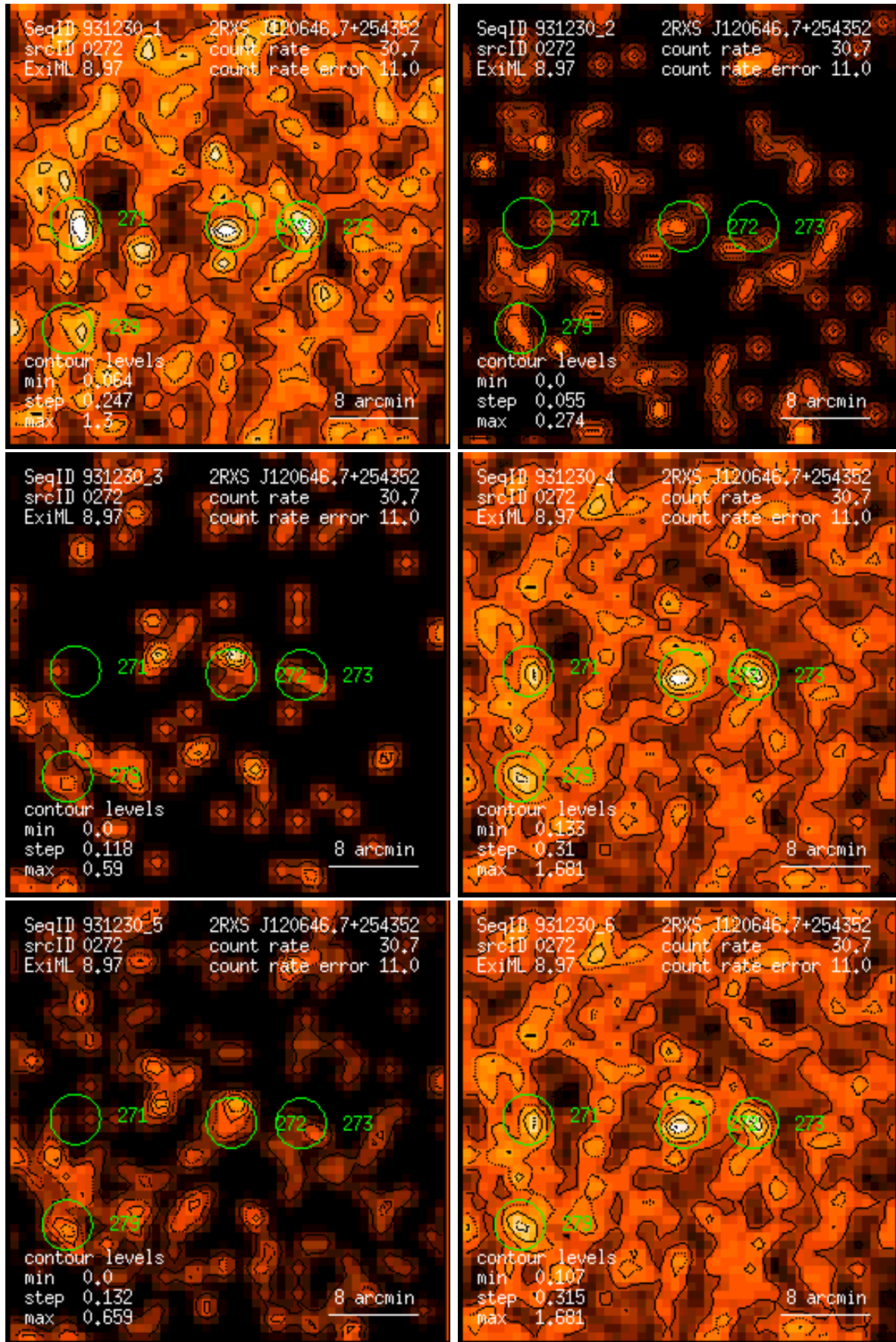
Figure 272: RASS 931230: detection 0272: band rate images, Gaussian filter: (1) PSPC channels 11 – 41, (2) 52 – 90, (3) 91 – 201, (4) 11 – 235, (5) 52 – 201, (6) 11 – 201. Broad band rates in counts/ks. Band rate contour levels in counts/ks/arcmin 2 .
