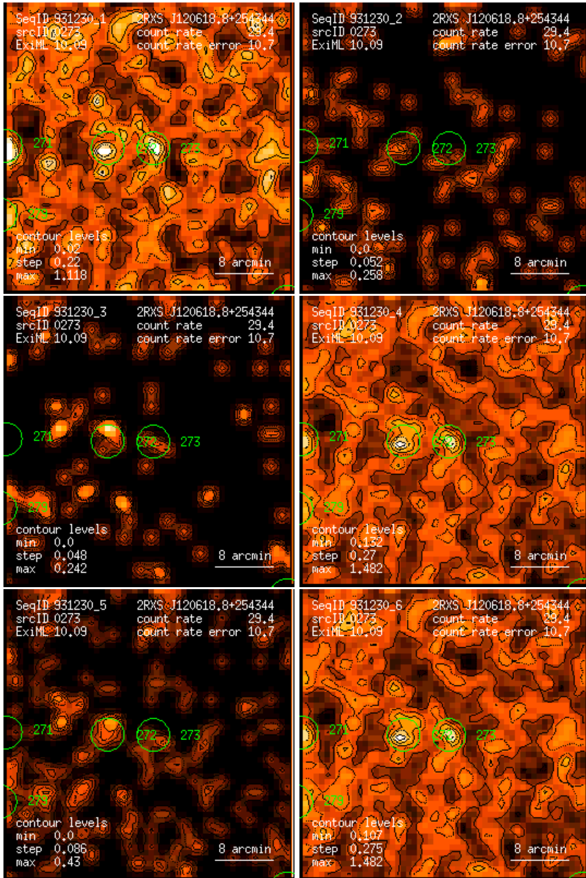
Figure 273: RASS 931230: detection 0273: band rate images, Gaussian filter: (1) PSPC channels 11 – 41, (2) 52 – 90, (3) 91 – 201, (4) 11 – 235, (5) 52 – 201, (6) 11 – 201. Broad band rates in counts/ks. Band rate contour levels in counts/ks/arcmin 2 .
