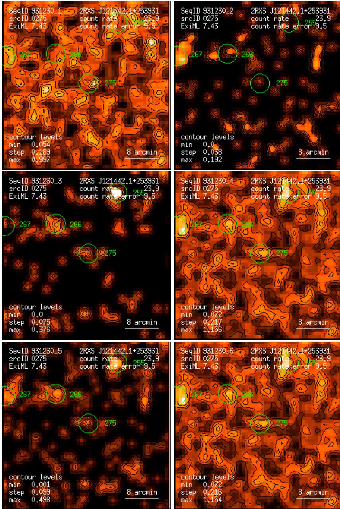
Figure 275: RASS 931230: detection 0275: band rate images, Gaussian filter: (1) PSPC channels 11 – 41, (2) 52 – 90, (3) 91 – 201, (4) 11 – 235, (5) 52 – 201, (6) 11 – 201. Broad band rates in counts/ks. Band rate contour levels in counts/ks/arcmin 2 .
