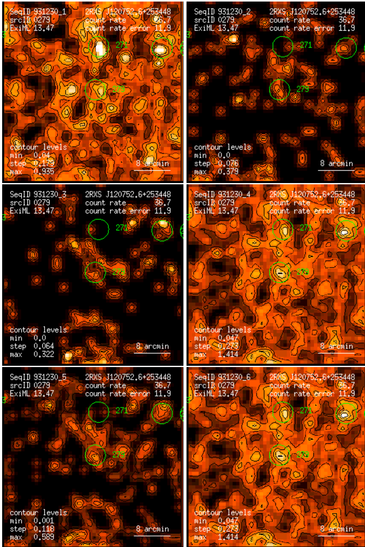
Figure 279: RASS 931230: detection 0279: band rate images, Gaussian filter: (1) PSPC channels 11 – 41, (2) 52 – 90, (3) 91 – 201, (4) 11 – 235, (5) 52 – 201, (6) 11 – 201. Broad band rates in counts/ks. Band rate contour levels in counts/ks/arcmin 2 .
