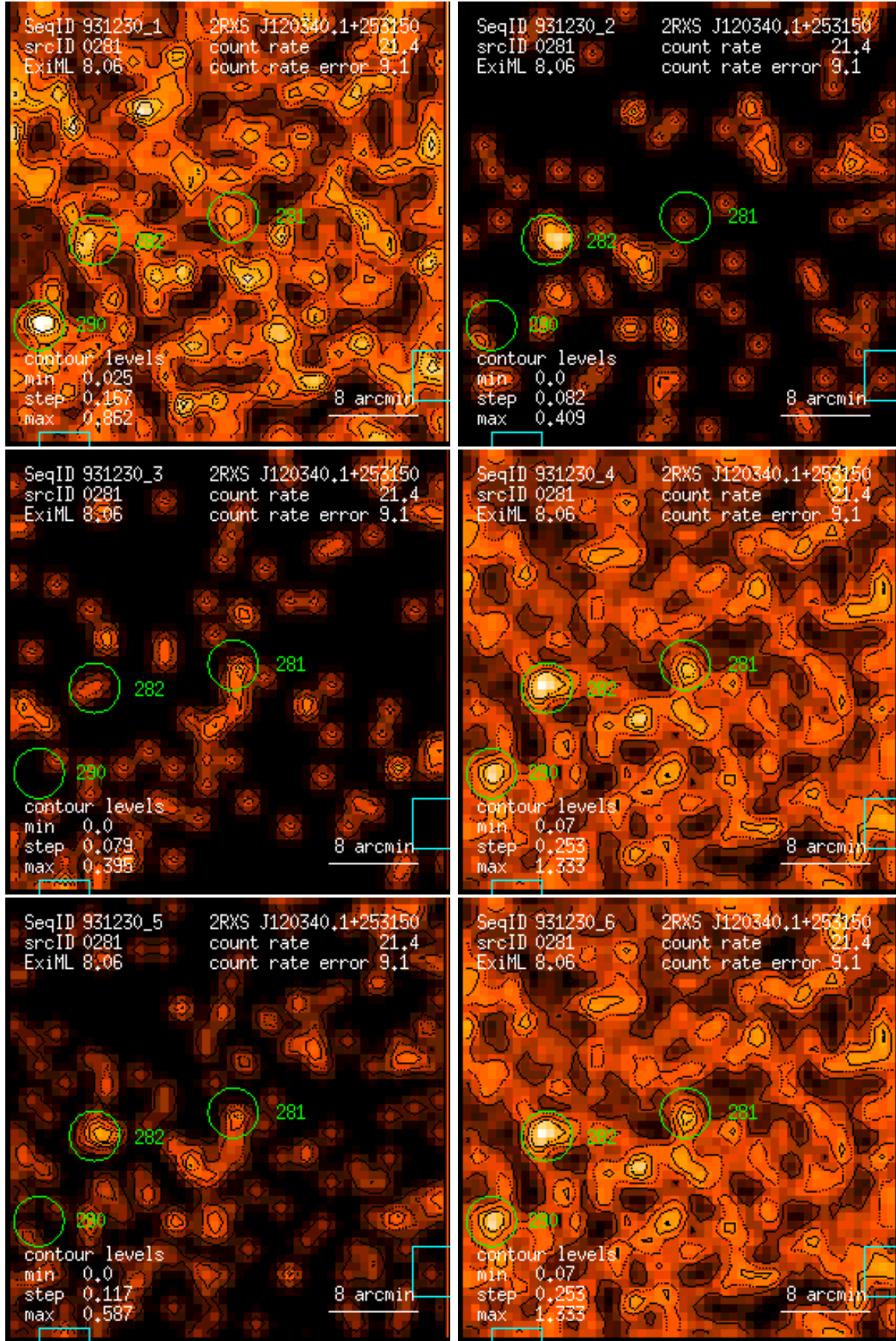
Figure 281: RASS 931230: detection 0281: band rate images, Gaussian filter: (1) PSPC channels 11 – 41, (2) 52 – 90, (3) 91 – 201, (4) 11 – 235, (5) 52 – 201, (6) 11 – 201. Broad band rates in counts/ks. Band rate contour levels in counts/ks/arcmin 2 .
