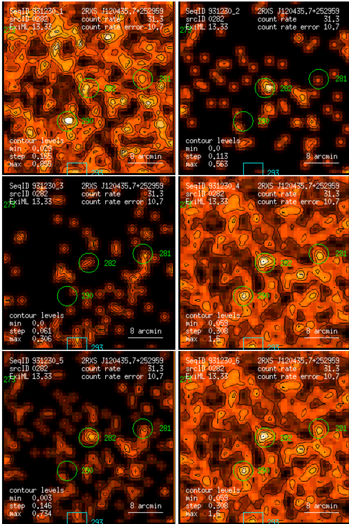
Figure 282: RASS 931230: detection 0282: band rate images, Gaussian filter: (1) PSPC channels 11 – 41, (2) 52 – 90, (3) 91 – 201, (4) 11 – 235, (5) 52 – 201, (6) 11 – 201. Broad band rates in counts/ks. Band rate contour levels in counts/ks/arcmin 2 .
