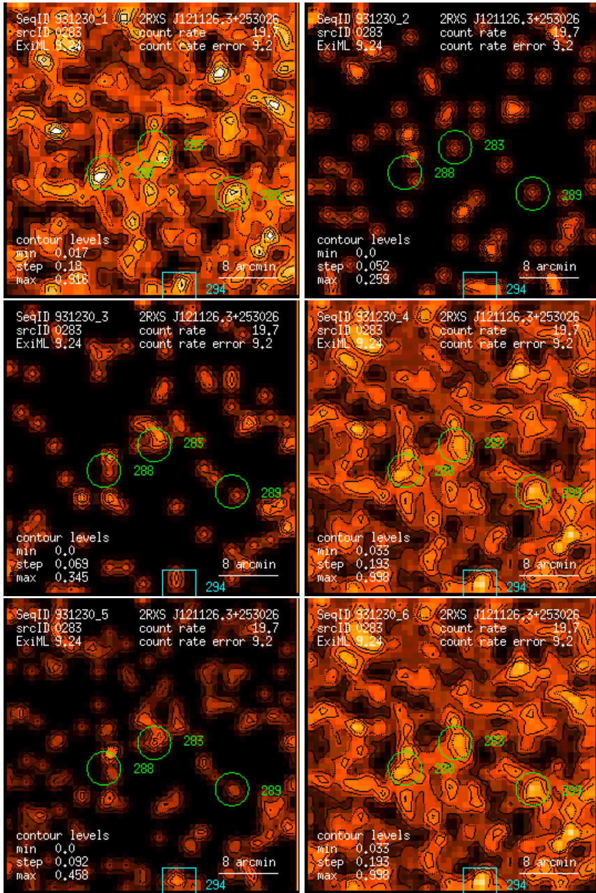
Figure 283: RASS 931230: detection 0283: band rate images, Gaussian filter: (1) PSPC channels 11 – 41, (2) 52 – 90, (3) 91 – 201, (4) 11 – 235, (5) 52 – 201, (6) 11 – 201. Broad band rates in counts/ks. Band rate contour levels in counts/ks/arcmin 2 .
