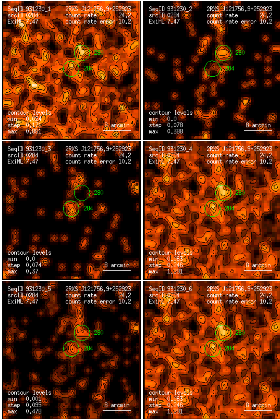
Figure 284: RASS 931230: detection 0284: band rate images, Gaussian filter: (1) PSPC channels 11 – 41, (2) 52 – 90, (3) 91 – 201, (4) 11 – 235, (5) 52 – 201, (6) 11 – 201. Broad band rates in counts/ks. Band rate contour levels in counts/ks/arcmin 2 .
