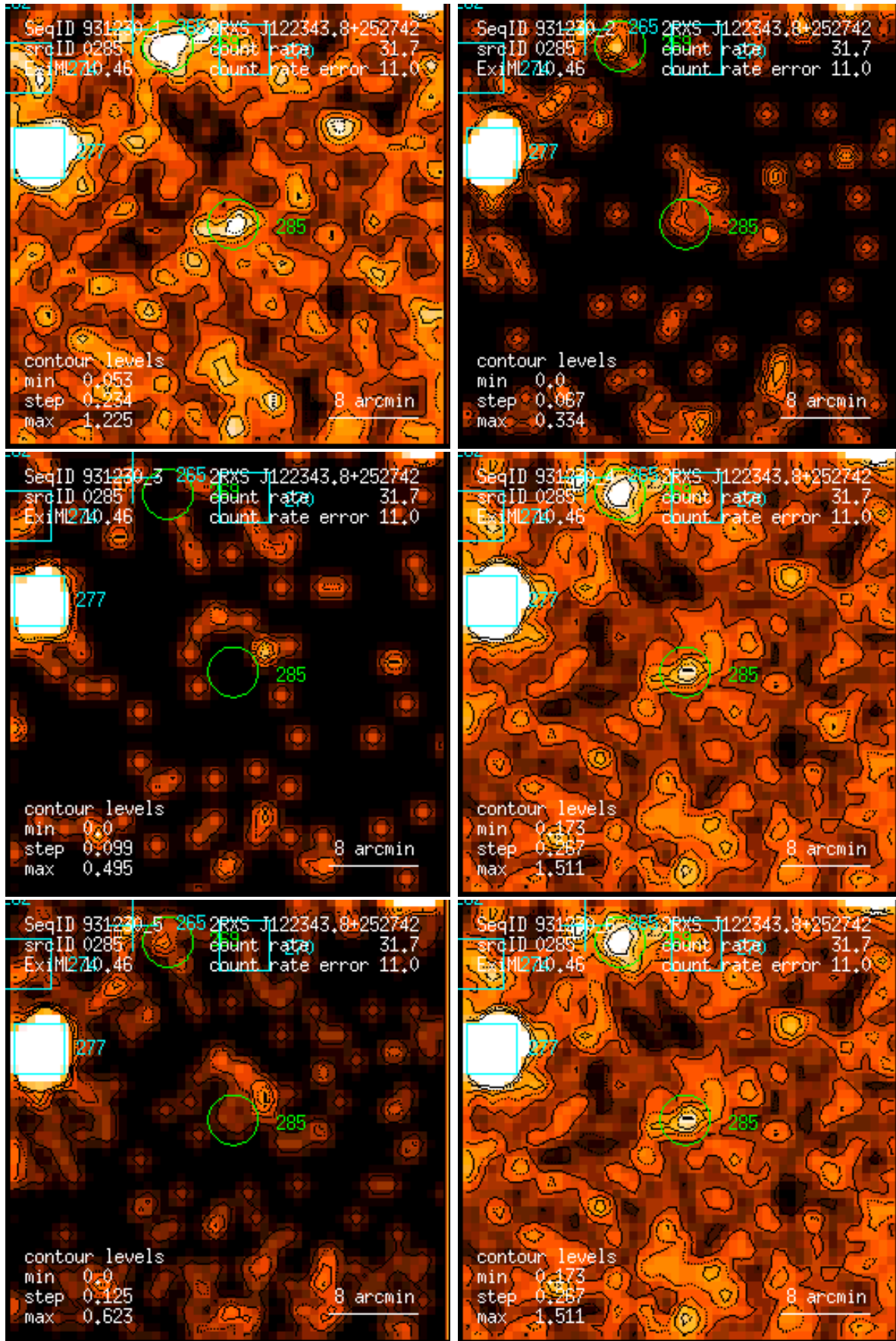
Figure 285: RASS 931230: detection 0285: band rate images, Gaussian filter: (1) PSPC channels 11 – 41, (2) 52 – 90, (3) 91 – 201, (4) 11 – 235, (5) 52 – 201, (6) 11 – 201. Broad band rates in counts/ks. Band rate contour levels in counts/ks/arcmin 2 .
