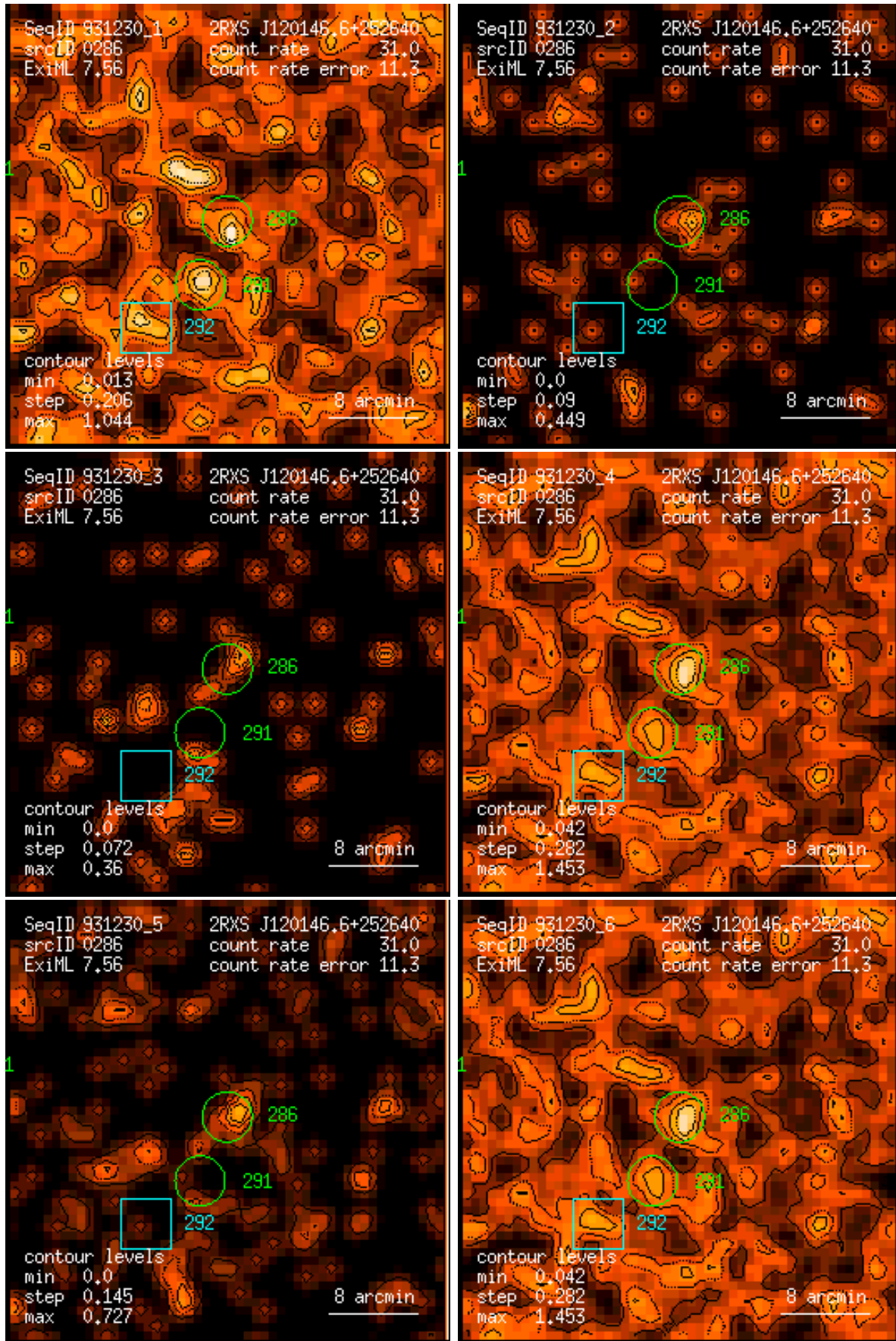
Figure 286: RASS 931230: detection 0286: band rate images, Gaussian filter: (1) PSPC channels 11 – 41, (2) 52 – 90, (3) 91 – 201, (4) 11 – 235, (5) 52 – 201, (6) 11 – 201. Broad band rates in counts/ks. Band rate contour levels in counts/ks/arcmin 2 .
