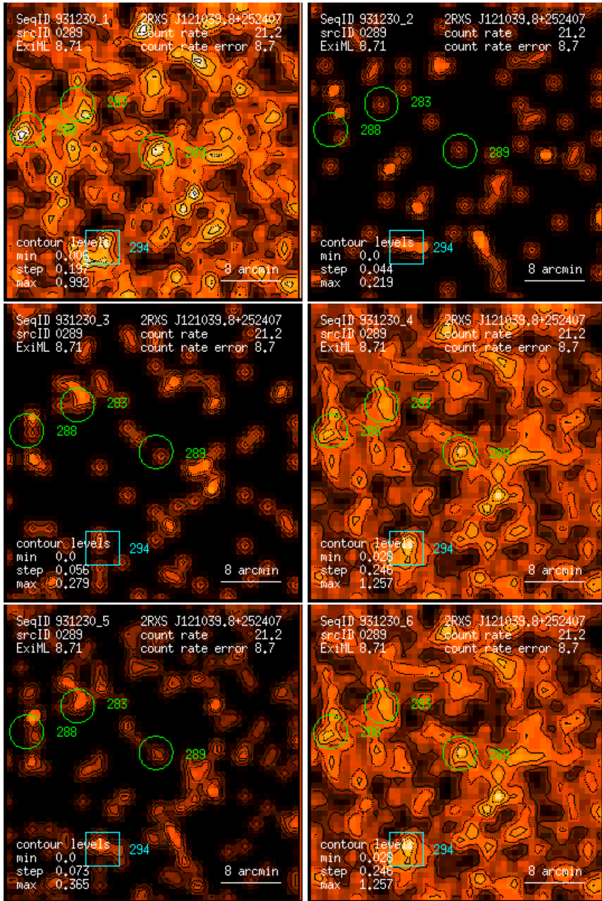
Figure 289: RASS 931230: detection 0289: band rate images, Gaussian filter: (1) PSPC channels 11 – 41, (2) 52 – 90, (3) 91 – 201, (4) 11 – 235, (5) 52 – 201, (6) 11 – 201. Broad band rates in counts/ks. Band rate contour levels in counts/ks/arcmin 2 .
