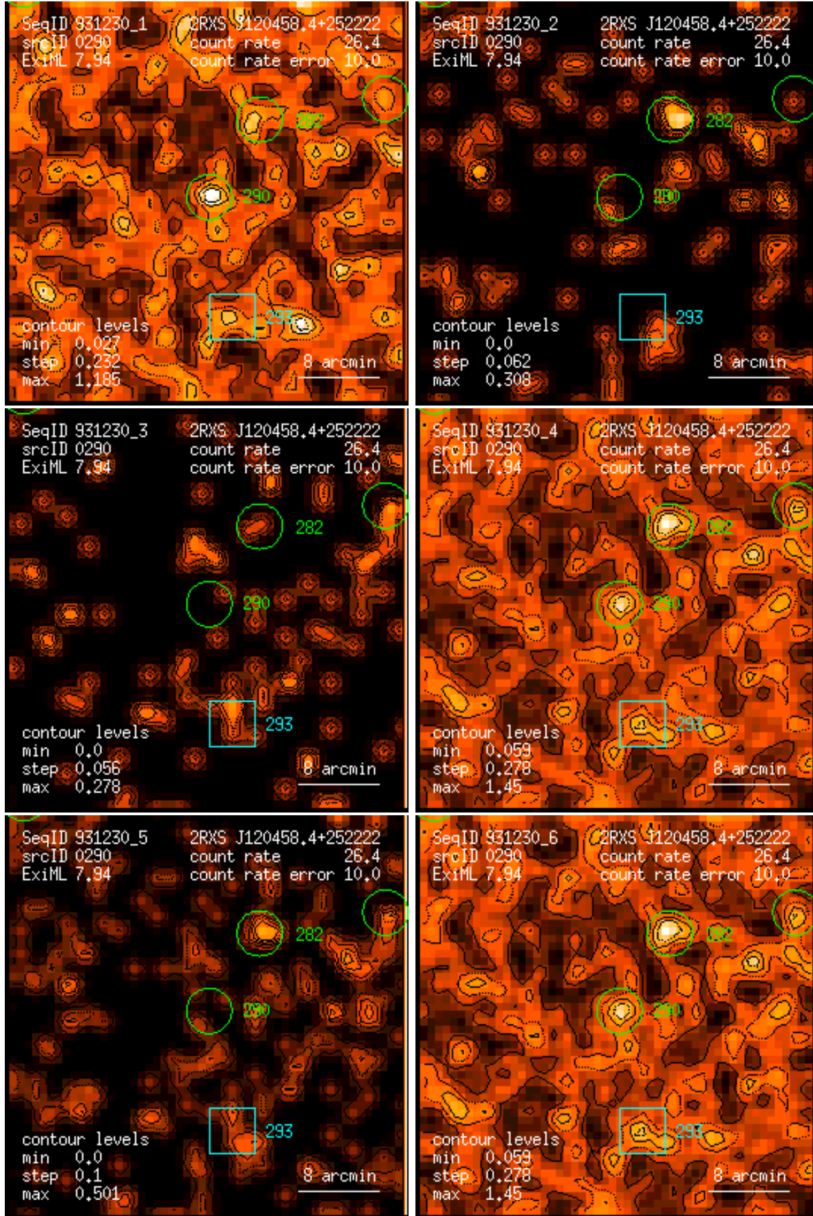
Figure 290: RASS 931230: detection 0290: band rate images, Gaussian filter: (1) PSPC channels 11 – 41, (2) 52 – 90, (3) 91 – 201, (4) 11 – 235, (5) 52 – 201, (6) 11 – 201. Broad band rates in counts/ks. Band rate contour levels in counts/ks/arcmin 2 .
