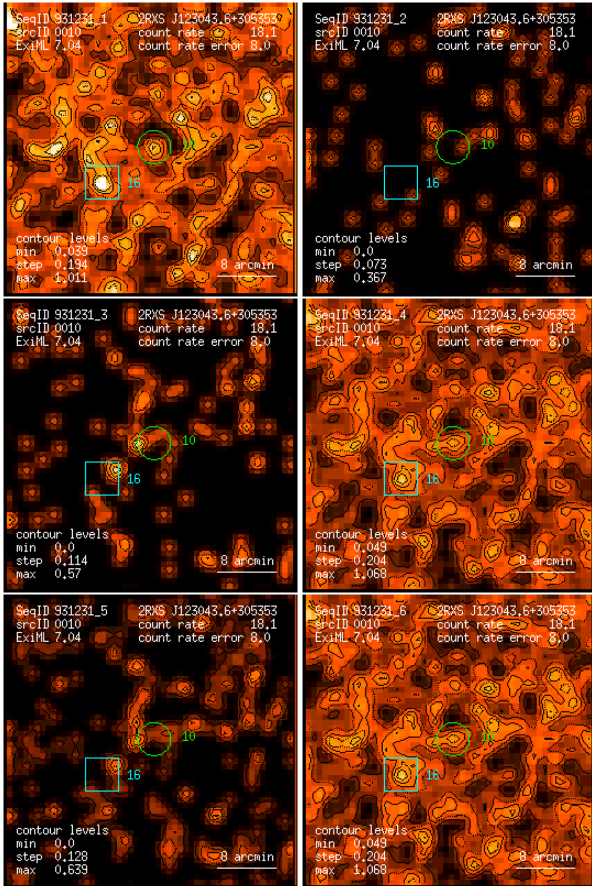
Figure 10: RASS 931231: detection 0010: band rate images, Gaussian filter: (1) PSPC channels 11 – 41, (2) 52 – 90, (3) 91 – 201, (4) 11 – 235, (5) 52 – 201, (6) 11 – 201. Broad band rates in counts/ks. Band rate contour levels in counts/ks/arcmin 2 .
