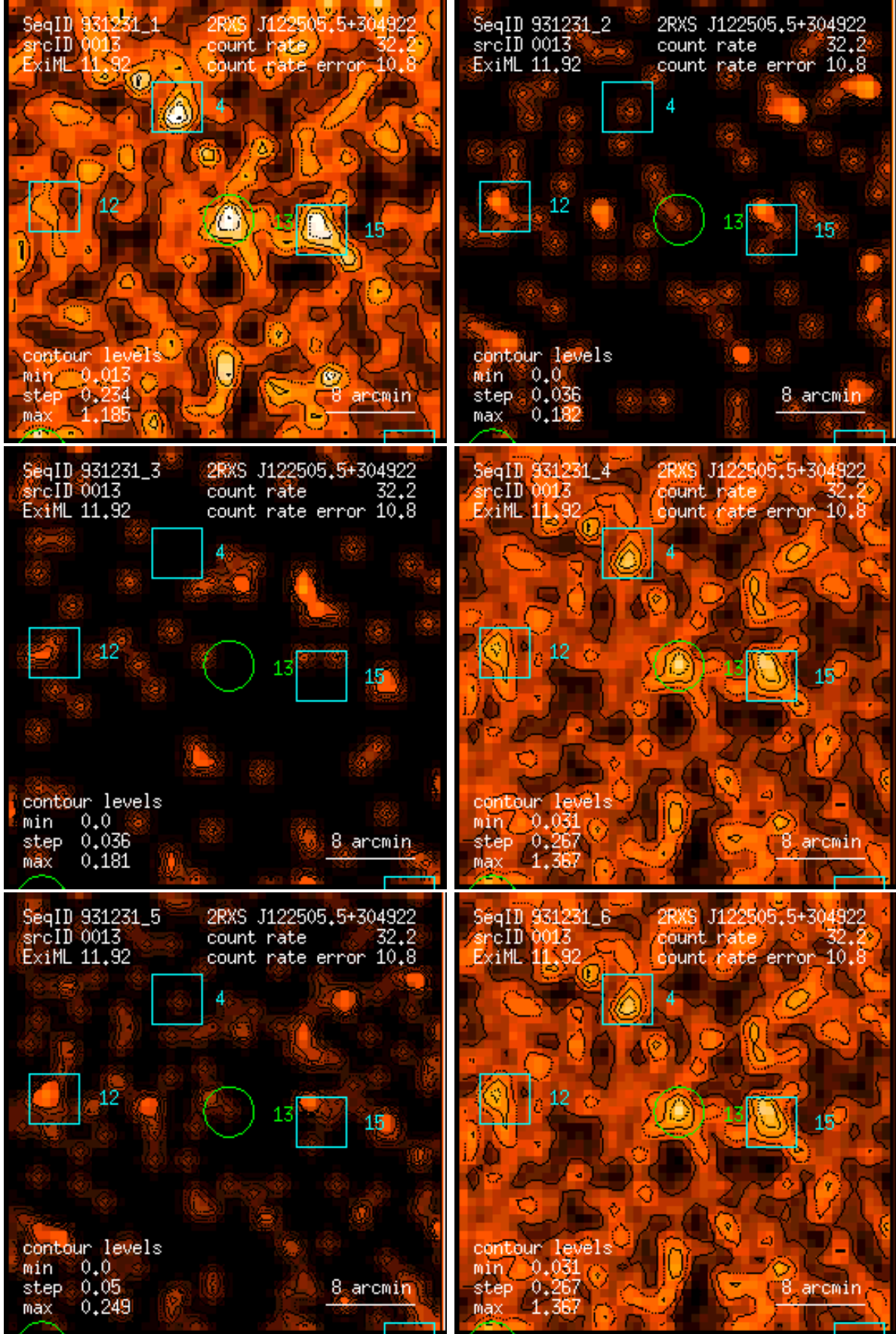
Figure 13: RASS 931231: detection 0013: band rate images, Gaussian filter: (1) PSPC channels 11 – 41, (2) 52 – 90, (3) 91 – 201, (4) 11 – 235, (5) 52 – 201, (6) 11 – 201. Broad band rates in counts/ks. Band rate contour levels in counts/ks/arcmin 2 .
