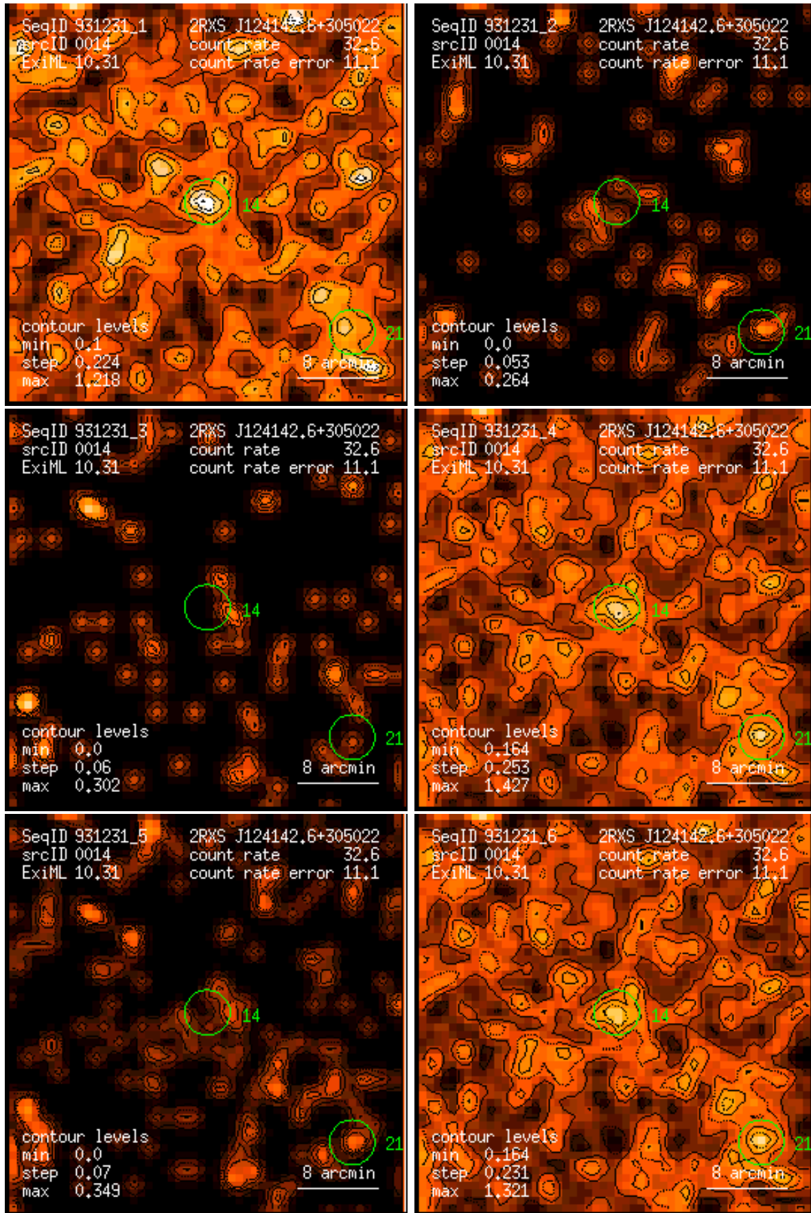
Figure 14: RASS 931231: detection 0014: band rate images, Gaussian filter: (1) PSPC channels 11 – 41, (2) 52 – 90, (3) 91 – 201, (4) 11 – 235, (5) 52 – 201, (6) 11 – 201. Broad band rates in counts/ks. Band rate contour levels in counts/ks/arcmin 2 .
