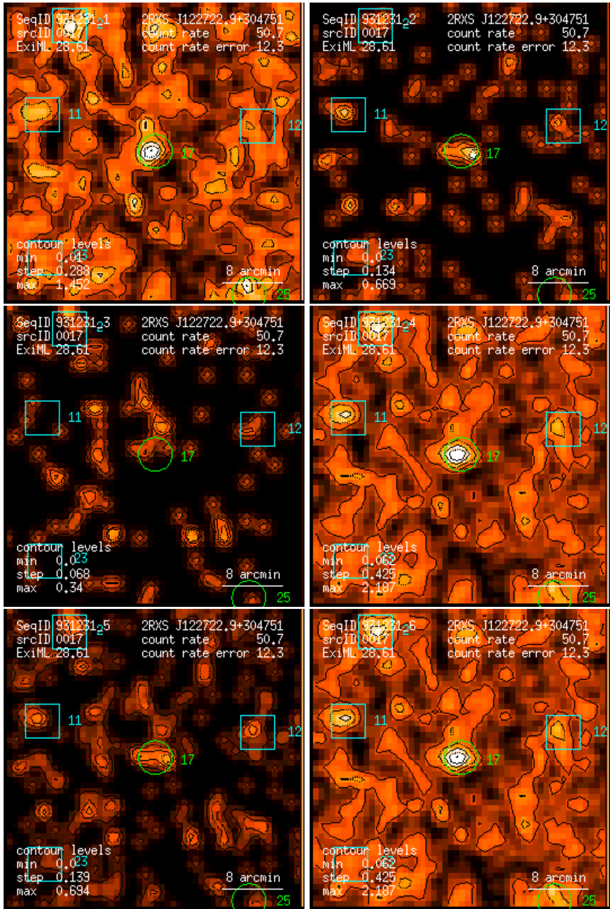
Figure 17: RASS 931231: detection 0017: band rate images, Gaussian filter: (1) PSPC channels 11 – 41, (2) 52 – 90, (3) 91 – 201, (4) 11 – 235, (5) 52 – 201, (6) 11 – 201. Broad band rates in counts/ks. Band rate contour levels in counts/ks/arcmin 2 .
