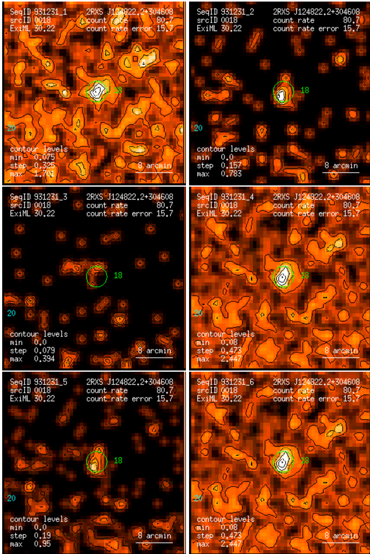
Figure 18: RASS 931231: detection 0018: band rate images, Gaussian filter: (1) PSPC channels 11 – 41, (2) 52 – 90, (3) 91 – 201, (4) 11 – 235, (5) 52 – 201, (6) 11 – 201. Broad band rates in counts/ks. Band rate contour levels in counts/ks/arcmin 2 .
