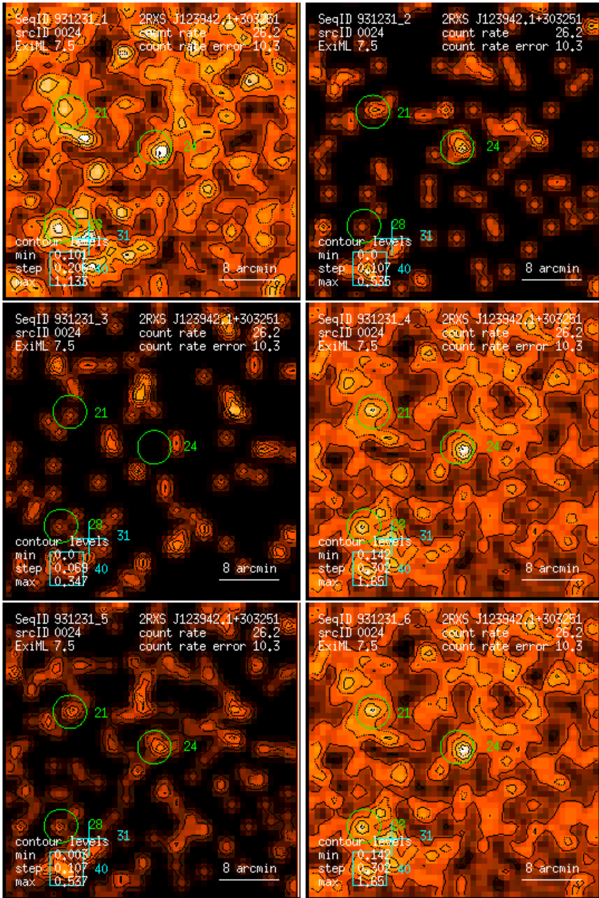
Figure 24: RASS 931231: detection 0024: band rate images, Gaussian filter: (1) PSPC channels 11 – 41, (2) 52 – 90, (3) 91 – 201, (4) 11 – 235, (5) 52 – 201, (6) 11 – 201. Broad band rates in counts/ks. Band rate contour levels in counts/ks/arcmin 2 .
