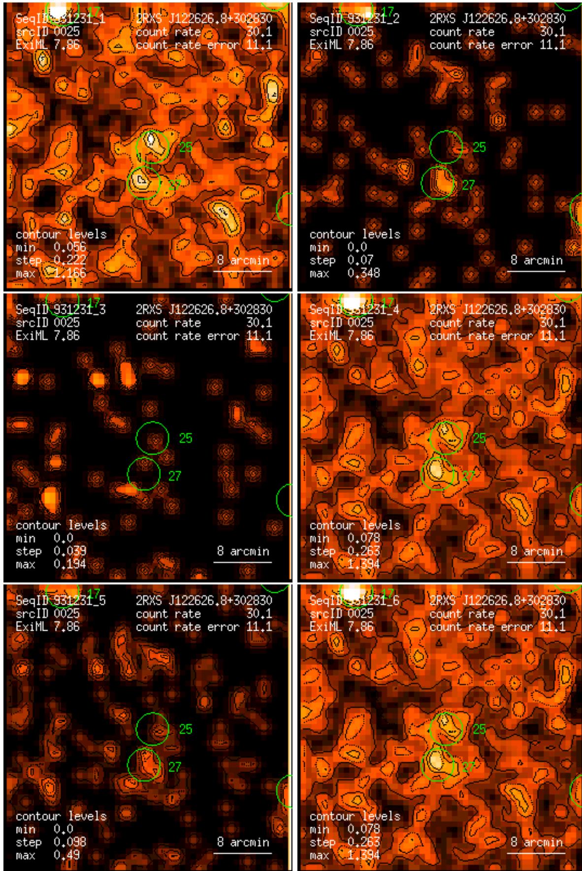
Figure 25: RASS 931231: detection 0025: band rate images, Gaussian filter: (1) PSPC channels 11 – 41, (2) 52 – 90, (3) 91 – 201, (4) 11 – 235, (5) 52 – 201, (6) 11 – 201. Broad band rates in counts/ks. Band rate contour levels in counts/ks/arcmin 2 .
