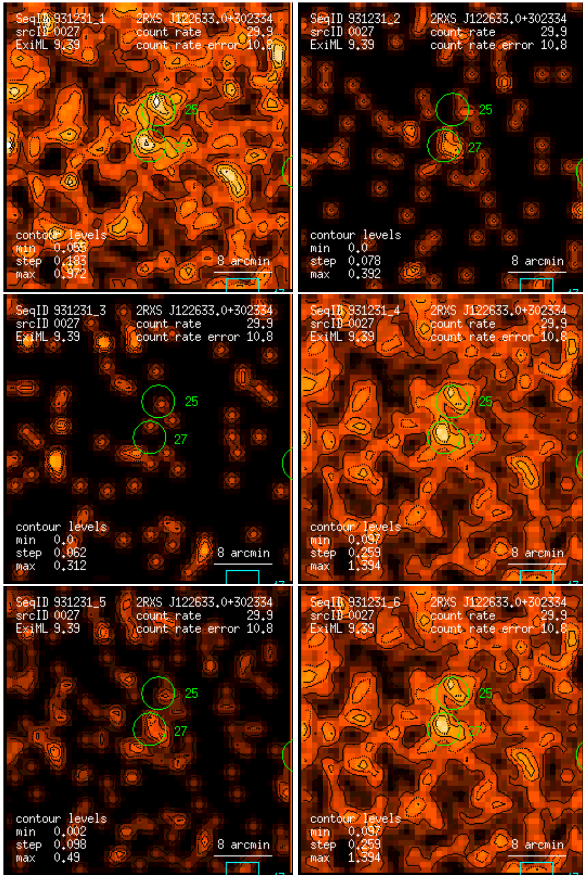
Figure 27: RASS 931231: detection 0027: band rate images, Gaussian filter: (1) PSPC channels 11 – 41, (2) 52 – 90, (3) 91 – 201, (4) 11 – 235, (5) 52 – 201, (6) 11 – 201. Broad band rates in counts/ks. Band rate contour levels in counts/ks/arcmin 2 .
