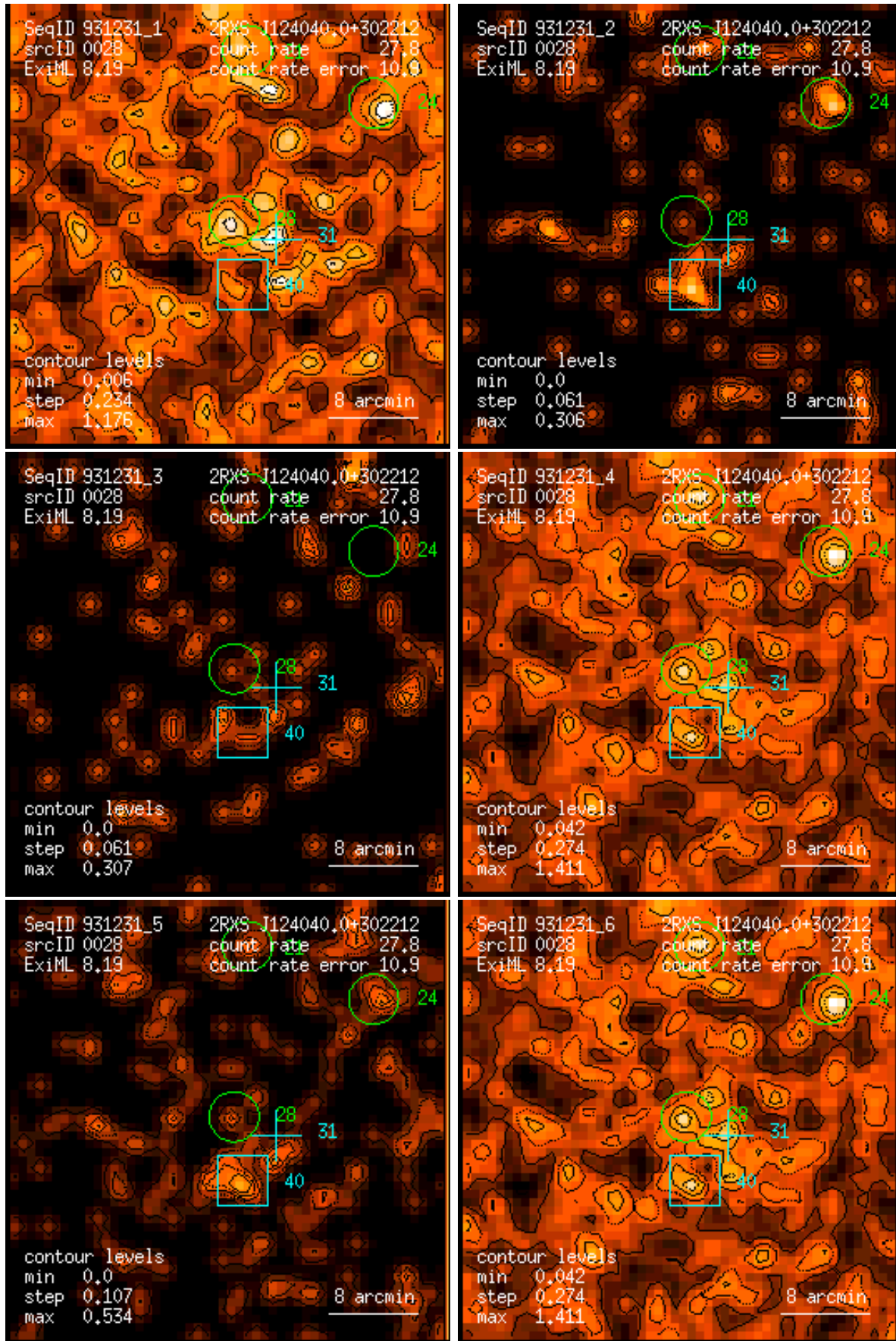
Figure 28: RASS 931231: detection 0028: band rate images, Gaussian filter: (1) PSPC channels 11 – 41, (2) 52 – 90, (3) 91 – 201, (4) 11 – 235, (5) 52 – 201, (6) 11 – 201. Broad band rates in counts/ks. Band rate contour levels in counts/ks/arcmin 2 .
