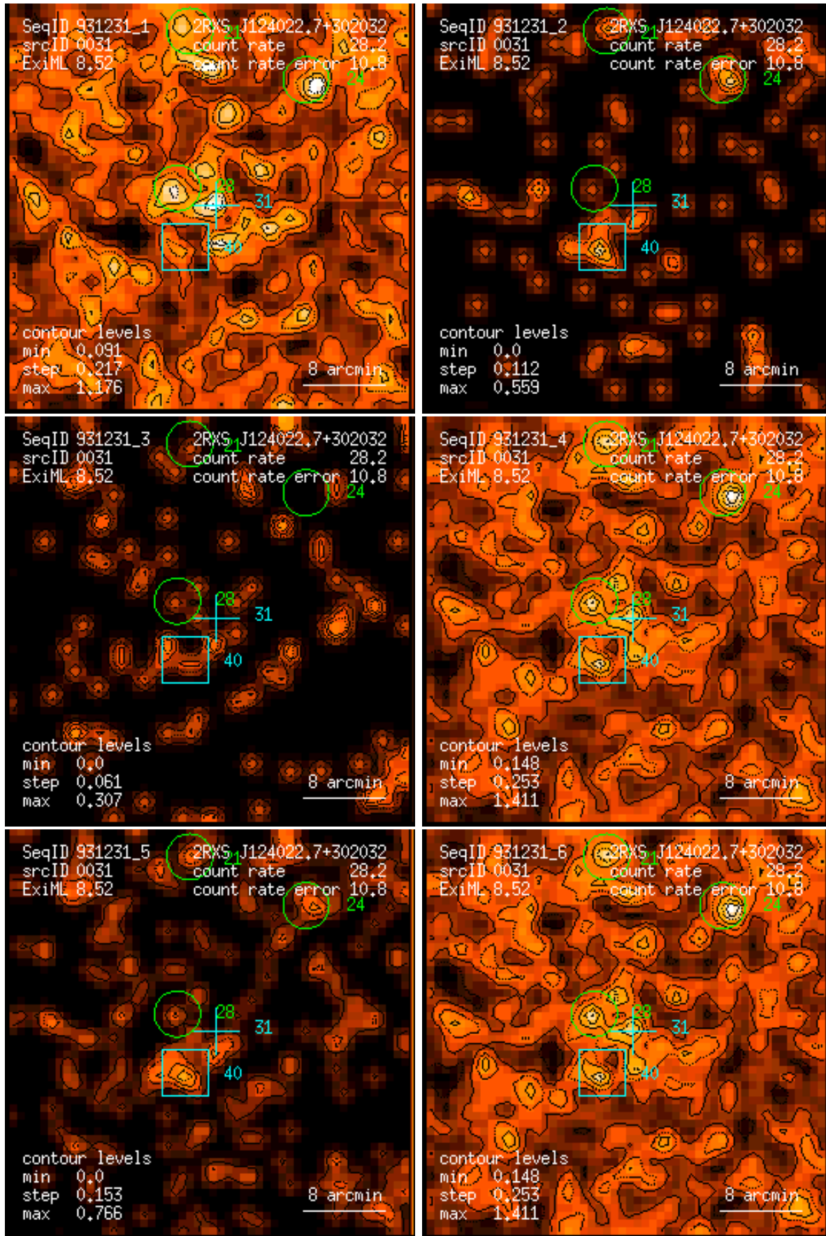
Figure 31: RASS 931231: detection 0031: band rate images, Gaussian filter: (1) PSPC channels 11 – 41, (2) 52 – 90, (3) 91 – 201, (4) 11 – 235, (5) 52 – 201, (6) 11 – 201. Broad band rates in counts/ks. Band rate contour levels in counts/ks/arcmin 2 .
