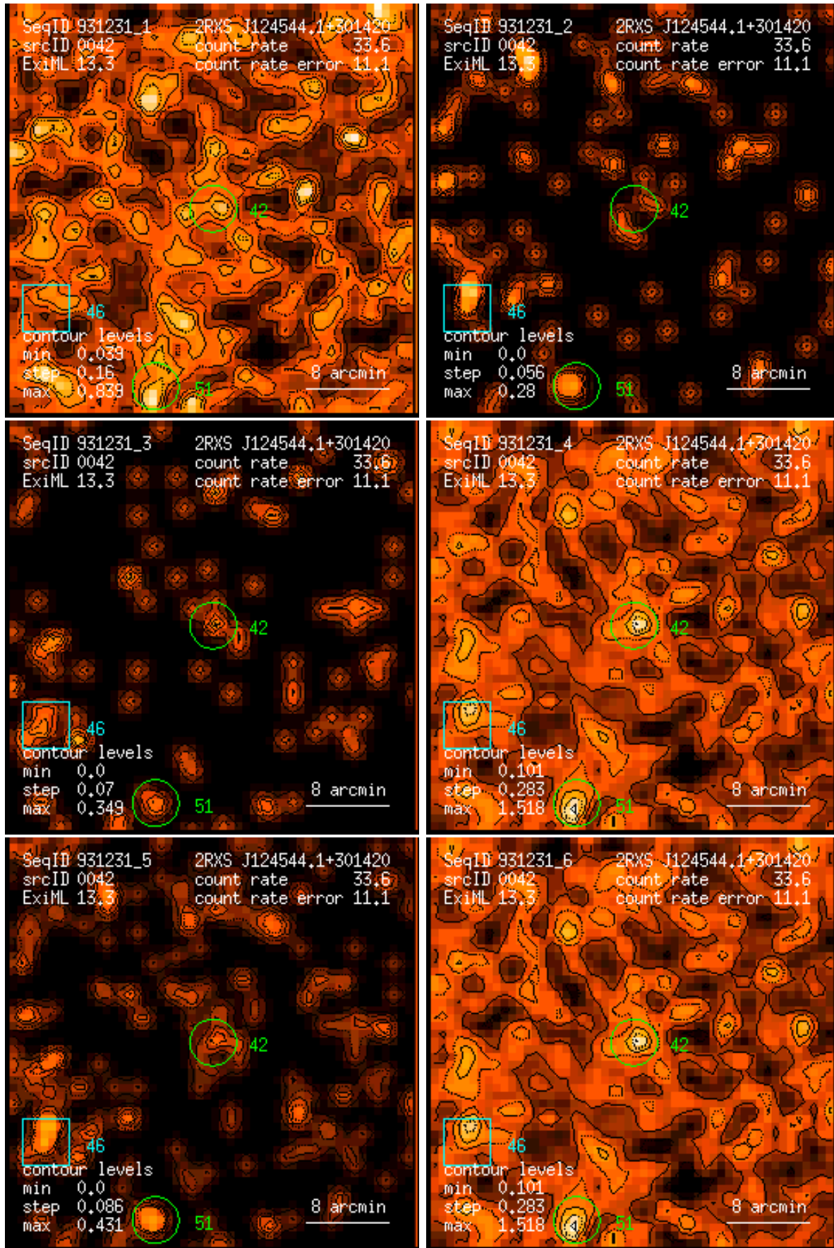
Figure 42: RASS 931231: detection 0042: band rate images, Gaussian filter: (1) PSPC channels 11 – 41, (2) 52 – 90, (3) 91 – 201, (4) 11 – 235, (5) 52 – 201, (6) 11 – 201. Broad band rates in counts/ks. Band rate contour levels in counts/ks/arcmin 2 .
