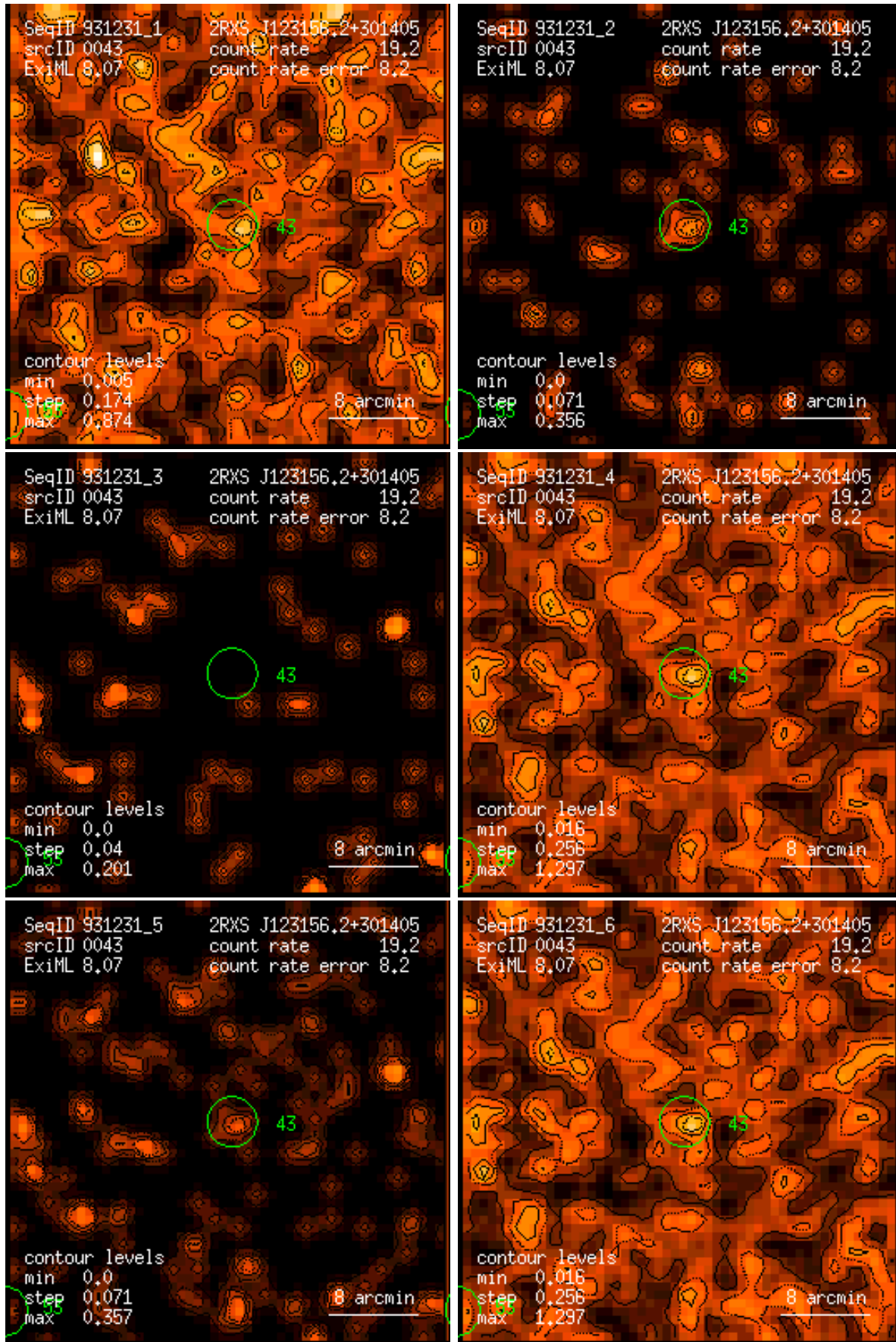
Figure 43: RASS 931231: detection 0043: band rate images, Gaussian filter: (1) PSPC channels 11 – 41, (2) 52 – 90, (3) 91 – 201, (4) 11 – 235, (5) 52 – 201, (6) 11 – 201. Broad band rates in counts/ks. Band rate contour levels in counts/ks/arcmin 2 .
