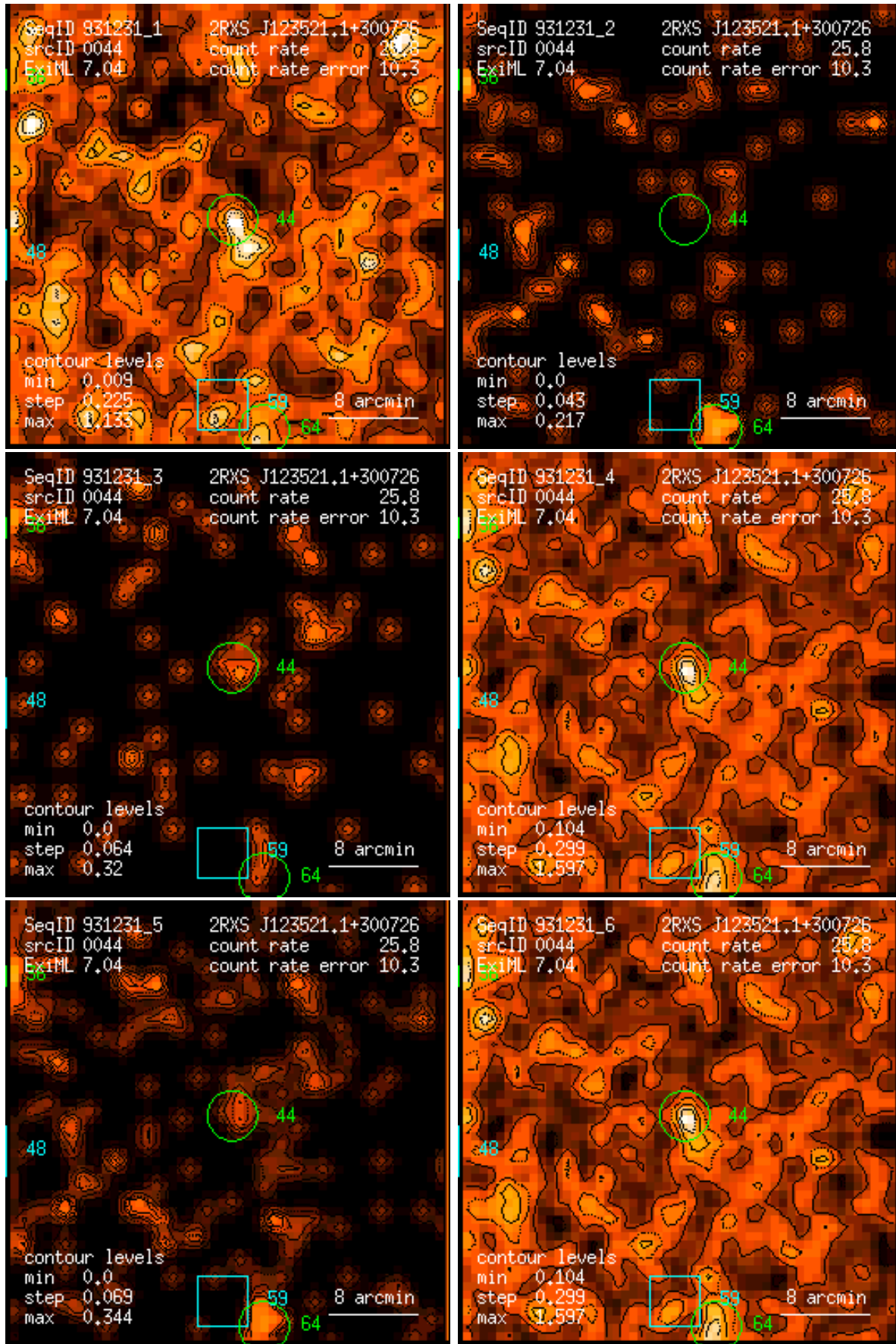
Figure 44: RASS 931231: detection 0044: band rate images, Gaussian filter: (1) PSPC channels 11 – 41, (2) 52 – 90, (3) 91 – 201, (4) 11 – 235, (5) 52 – 201, (6) 11 – 201. Broad band rates in counts/ks. Band rate contour levels in counts/ks/arcmin 2 .
