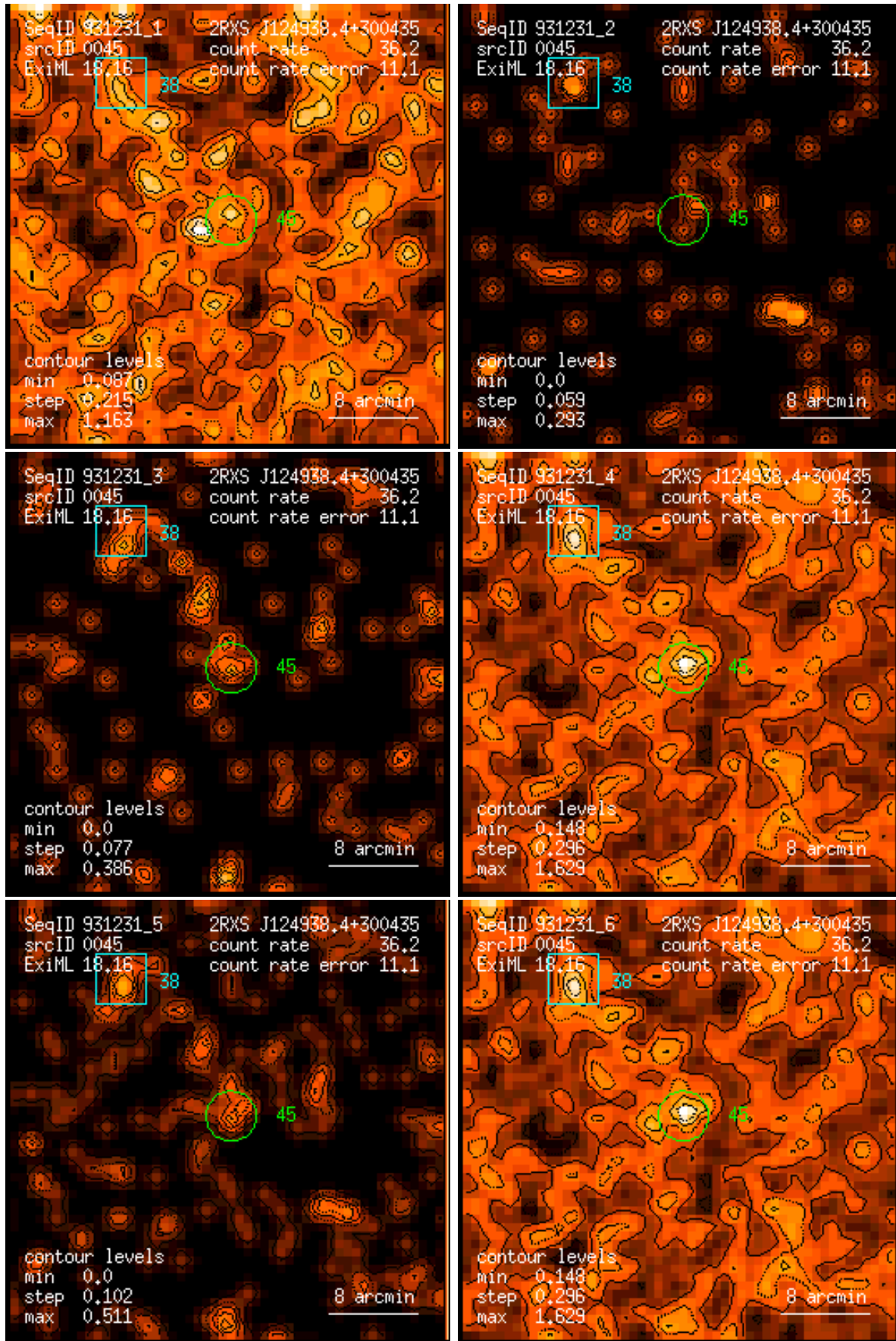
Figure 45: RASS 931231: detection 0045: band rate images, Gaussian filter: (1) PSPC channels 11 – 41, (2) 52 – 90, (3) 91 – 201, (4) 11 – 235, (5) 52 – 201, (6) 11 – 201. Broad band rates in counts/ks. Band rate contour levels in counts/ks/arcmin 2 .
