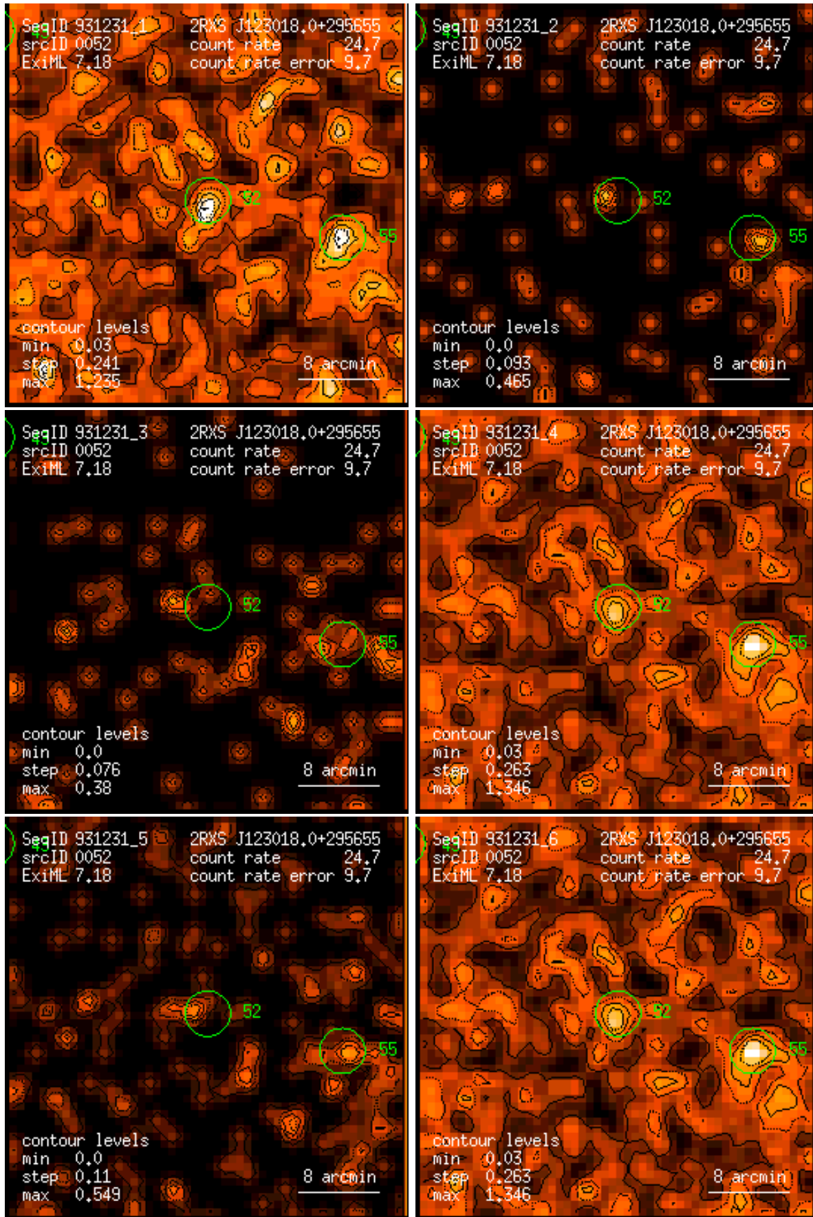
Figure 52: RASS 931231: detection 0052: band rate images, Gaussian filter: (1) PSPC channels 11 – 41, (2) 52 – 90, (3) 91 – 201, (4) 11 – 235, (5) 52 – 201, (6) 11 – 201. Broad band rates in counts/ks. Band rate contour levels in counts/ks/arcmin 2 .
