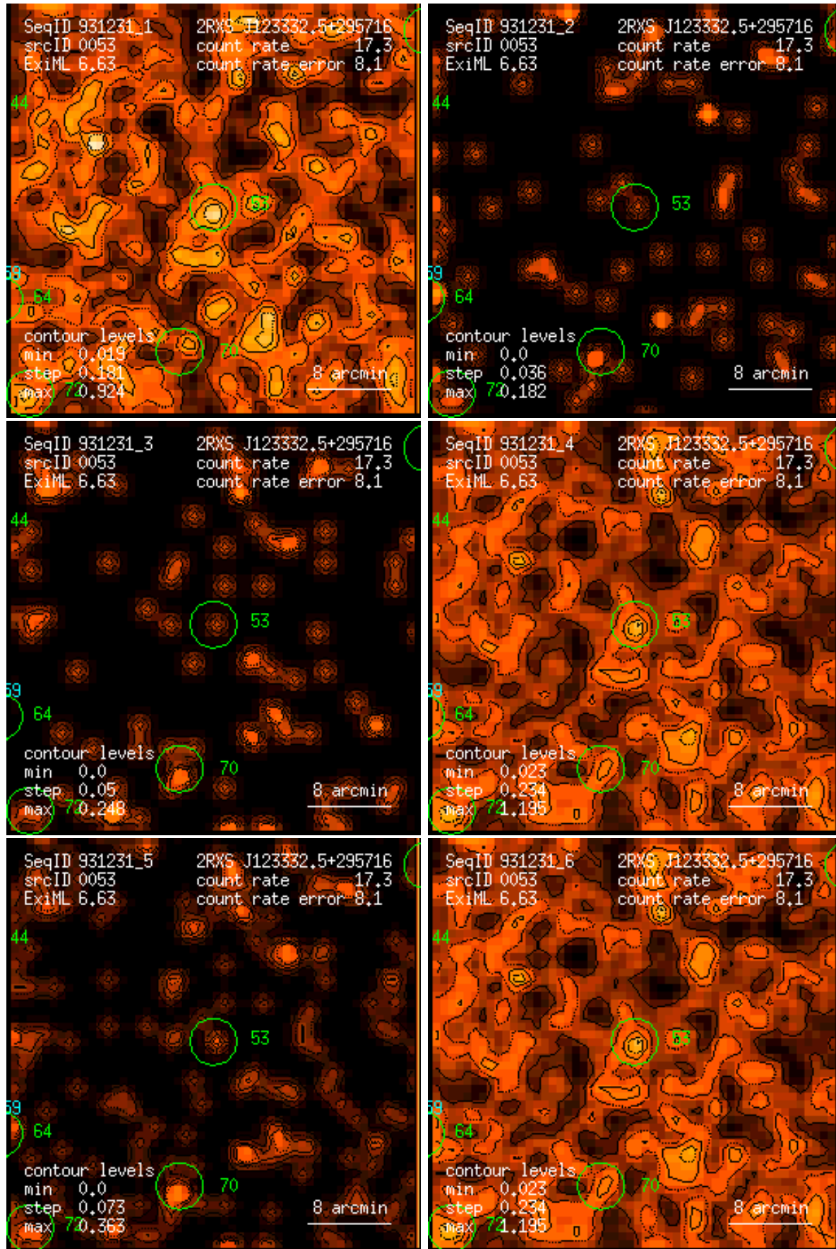
Figure 53: RASS 931231: detection 0053: band rate images, Gaussian filter: (1) PSPC channels 11 – 41, (2) 52 – 90, (3) 91 – 201, (4) 11 – 235, (5) 52 – 201, (6) 11 – 201. Broad band rates in counts/ks. Band rate contour levels in counts/ks/arcmin 2 .
