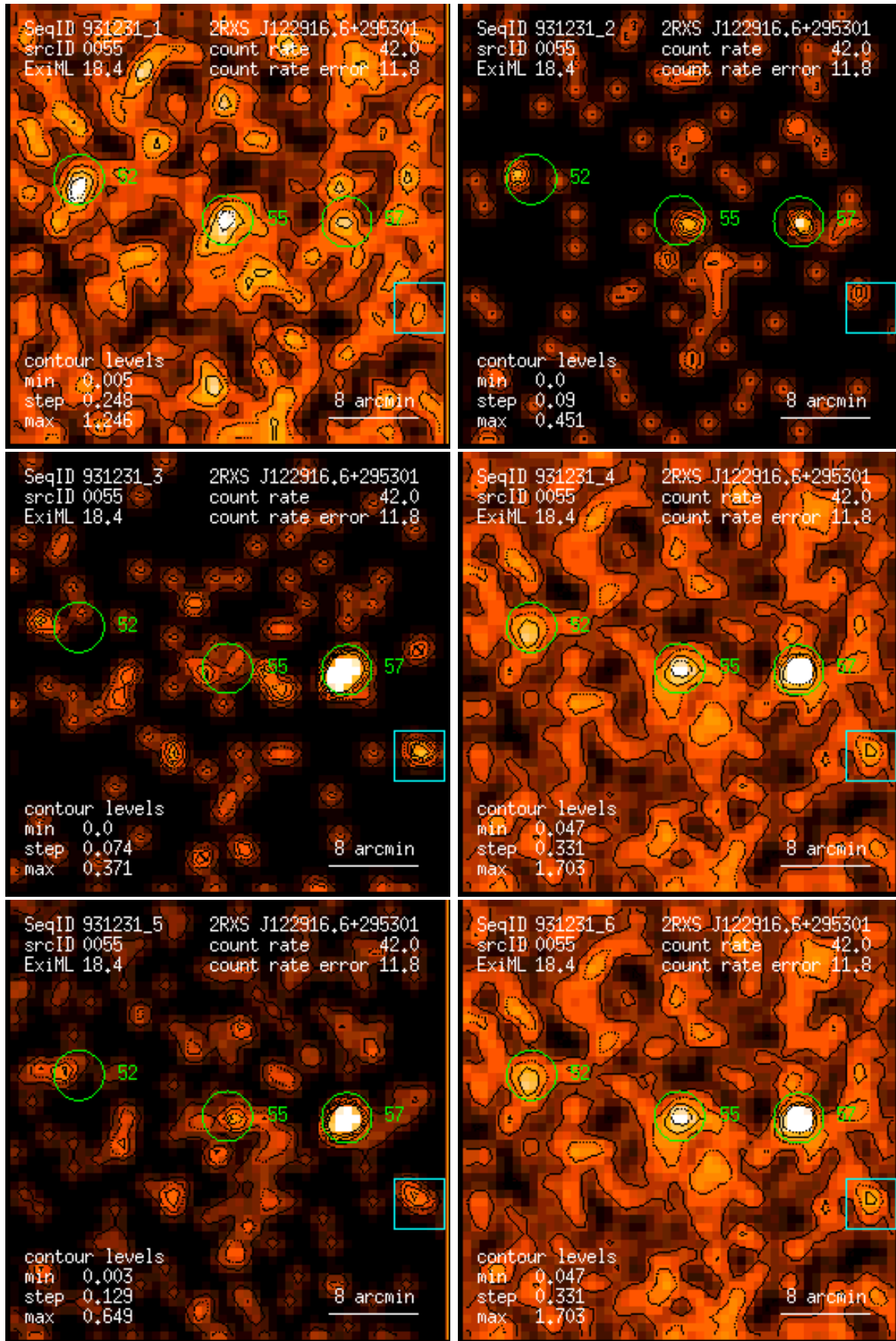
Figure 55: RASS 931231: detection 0055: band rate images, Gaussian filter: (1) PSPC channels 11 – 41, (2) 52 – 90, (3) 91 – 201, (4) 11 – 235, (5) 52 – 201, (6) 11 – 201. Broad band rates in counts/ks. Band rate contour levels in counts/ks/arcmin 2 .
