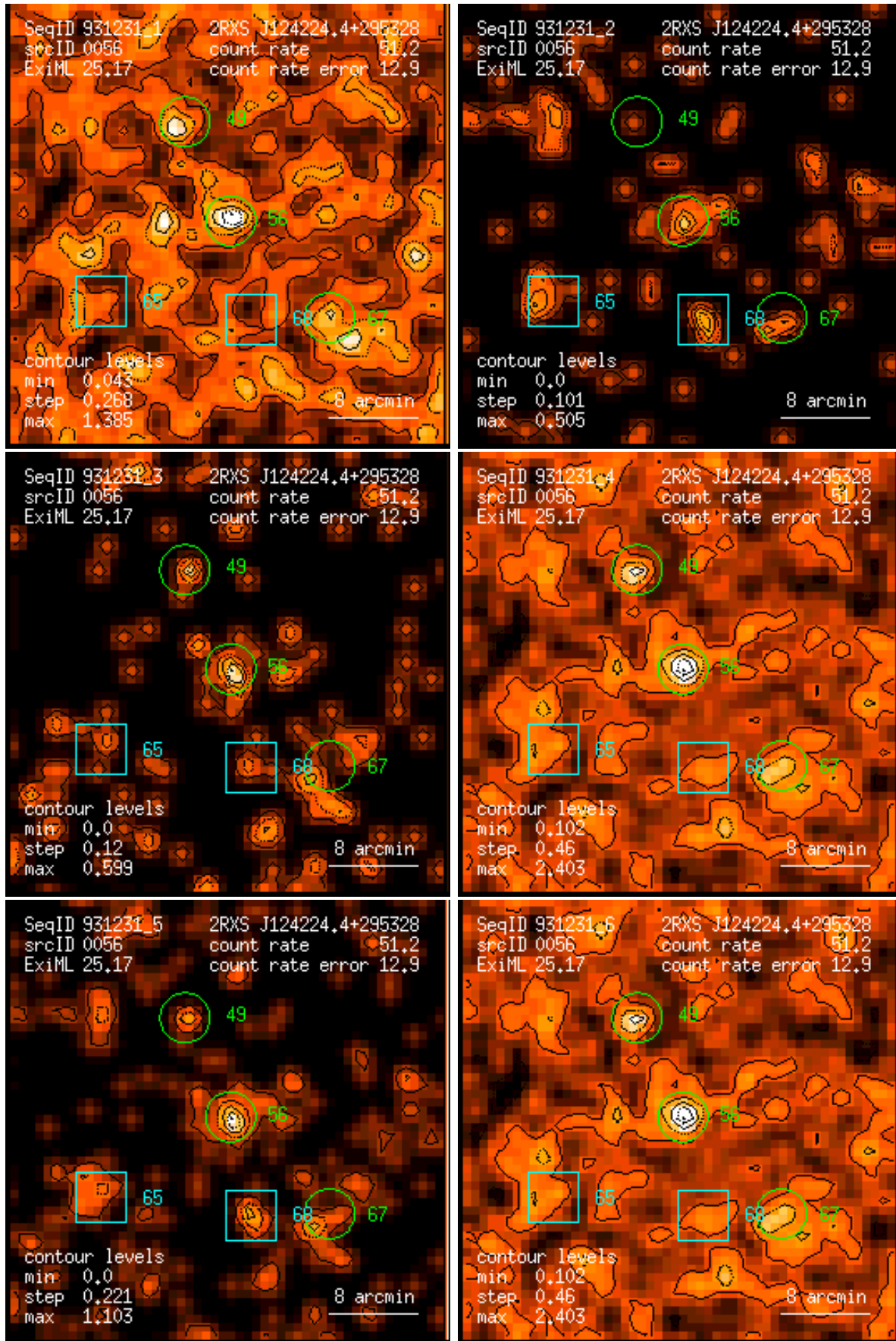
Figure 56: RASS 931231: detection 0056: band rate images, Gaussian filter: (1) PSPC channels 11 – 41, (2) 52 – 90, (3) 91 – 201, (4) 11 – 235, (5) 52 – 201, (6) 11 – 201. Broad band rates in counts/ks. Band rate contour levels in counts/ks/arcmin 2 .
