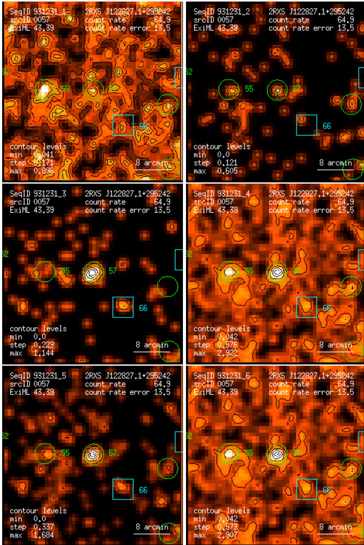
Figure 57: RASS 931231: detection 0057: band rate images, Gaussian filter: (1) PSPC channels 11 – 41, (2) 52 – 90, (3) 91 – 201, (4) 11 – 235, (5) 52 – 201, (6) 11 – 201. Broad band rates in counts/ks. Band rate contour levels in counts/ks/arcmin 2 .
