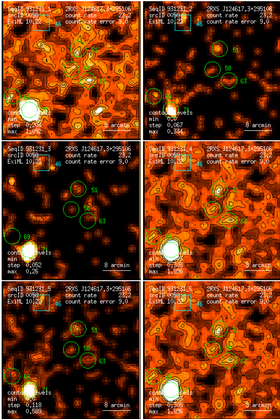
Figure 58: RASS 931231: detection 0058: band rate images, Gaussian filter: (1) PSPC channels 11 – 41, (2) 52 – 90, (3) 91 – 201, (4) 11 – 235, (5) 52 – 201, (6) 11 – 201. Broad band rates in counts/ks. Band rate contour levels in counts/ks/arcmin 2 .
