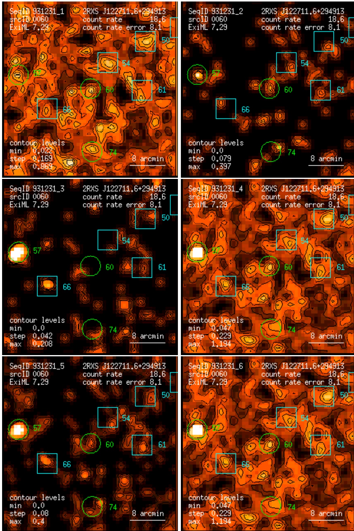
Figure 60: RASS 931231: detection 0060: band rate images, Gaussian filter: (1) PSPC channels 11 – 41, (2) 52 – 90, (3) 91 – 201, (4) 11 – 235, (5) 52 – 201, (6) 11 – 201. Broad band rates in counts/ks. Band rate contour levels in counts/ks/arcmin 2 .
