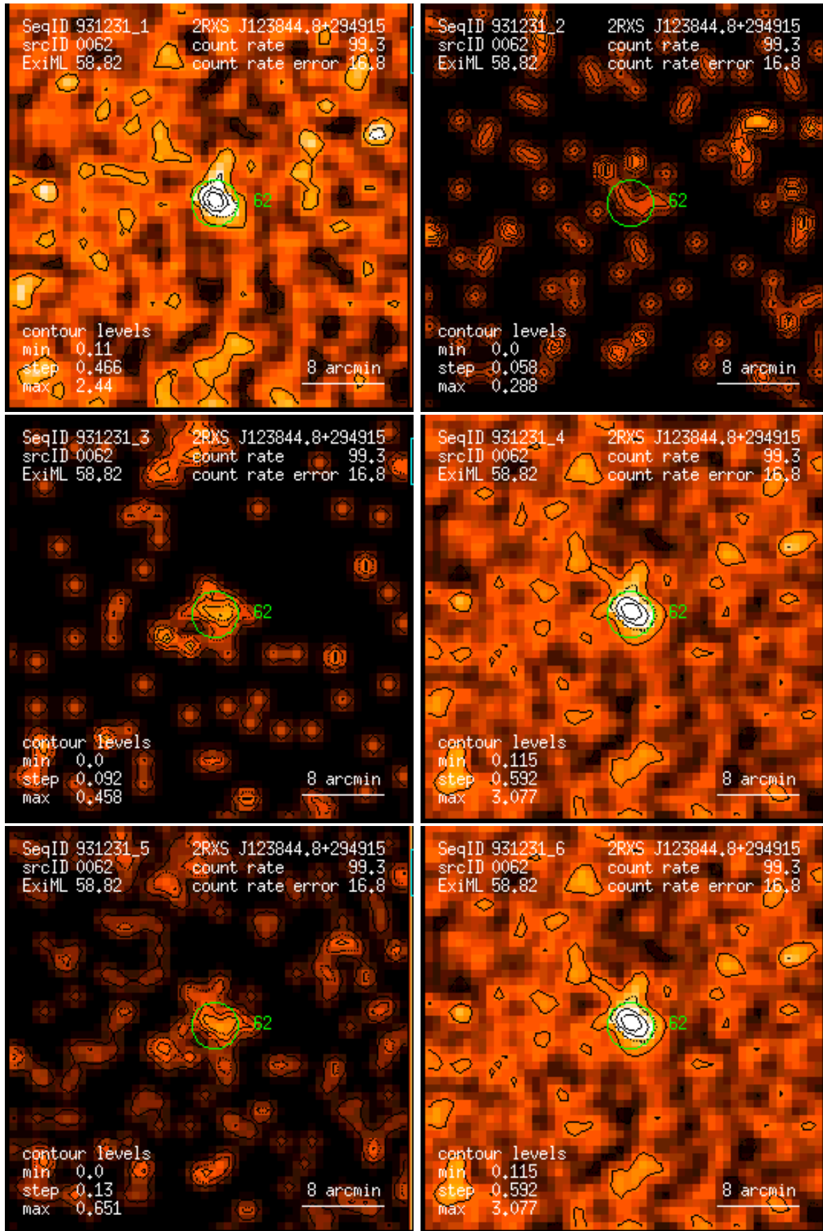
Figure 62: RASS 931231: detection 0062: band rate images, Gaussian filter: (1) PSPC channels 11 – 41, (2) 52 – 90, (3) 91 – 201, (4) 11 – 235, (5) 52 – 201, (6) 11 – 201. Broad band rates in counts/ks. Band rate contour levels in counts/ks/arcmin 2 .
