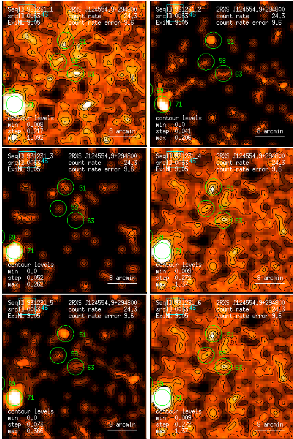
Figure 63: RASS 931231: detection 0063: band rate images, Gaussian filter: (1) PSPC channels 11 – 41, (2) 52 – 90, (3) 91 – 201, (4) 11 – 235, (5) 52 – 201, (6) 11 – 201. Broad band rates in counts/ks. Band rate contour levels in counts/ks/arcmin 2 .
