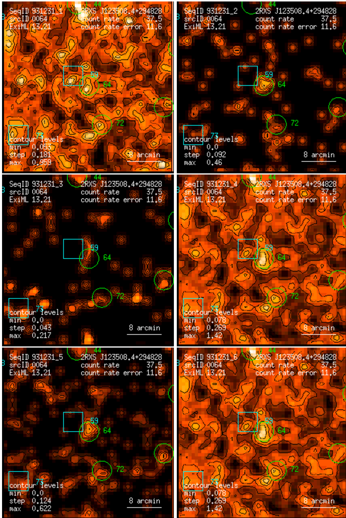
Figure 64: RASS 931231: detection 0064: band rate images, Gaussian filter: (1) PSPC channels 11 – 41, (2) 52 – 90, (3) 91 – 201, (4) 11 – 235, (5) 52 – 201, (6) 11 – 201. Broad band rates in counts/ks. Band rate contour levels in counts/ks/arcmin 2 .
