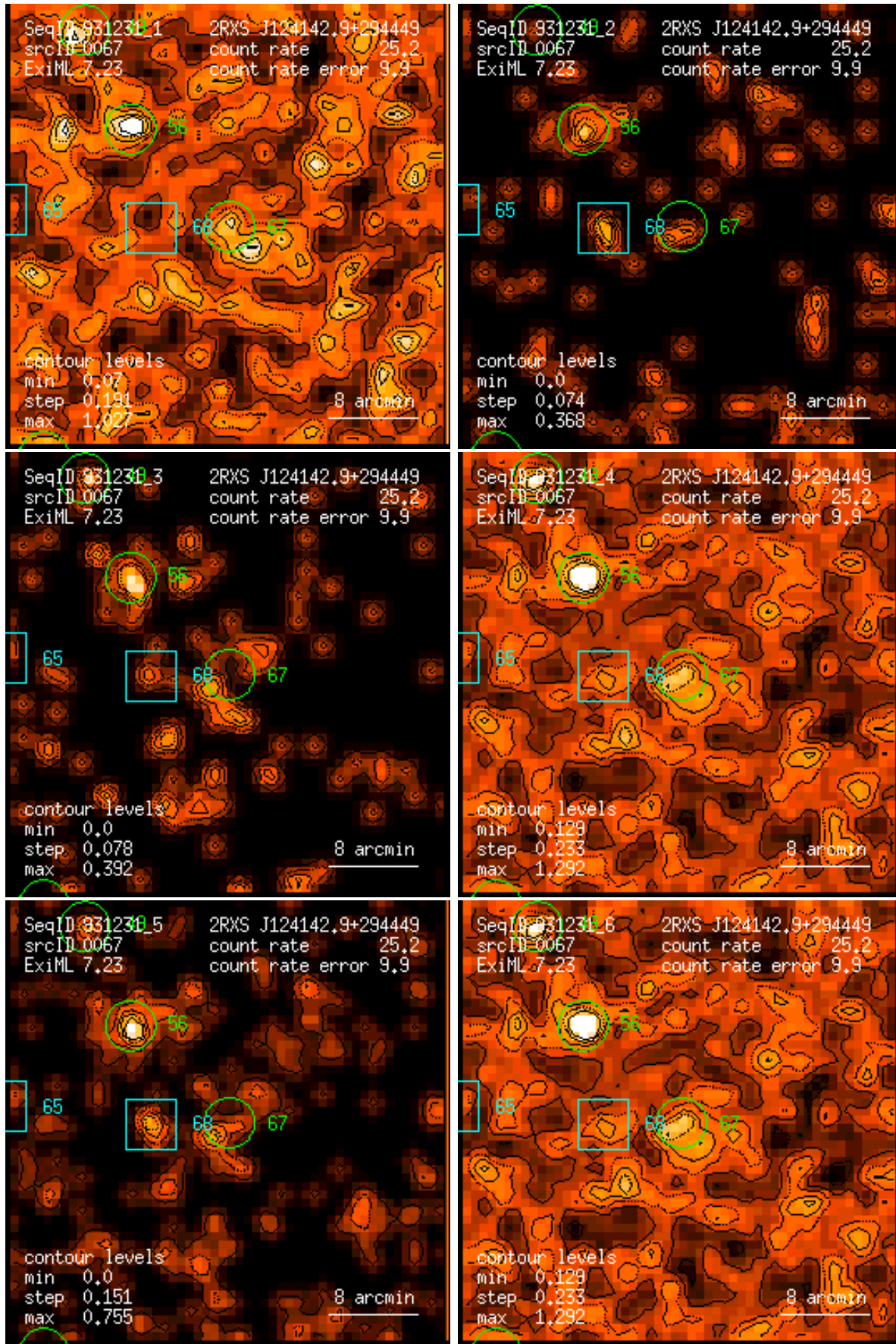
Figure 67: RASS 931231: detection 0067: band rate images, Gaussian filter: (1) PSPC channels 11 – 41, (2) 52 – 90, (3) 91 – 201, (4) 11 – 235, (5) 52 – 201, (6) 11 – 201. Broad band rates in counts/ks. Band rate contour levels in counts/ks/arcmin 2 .
