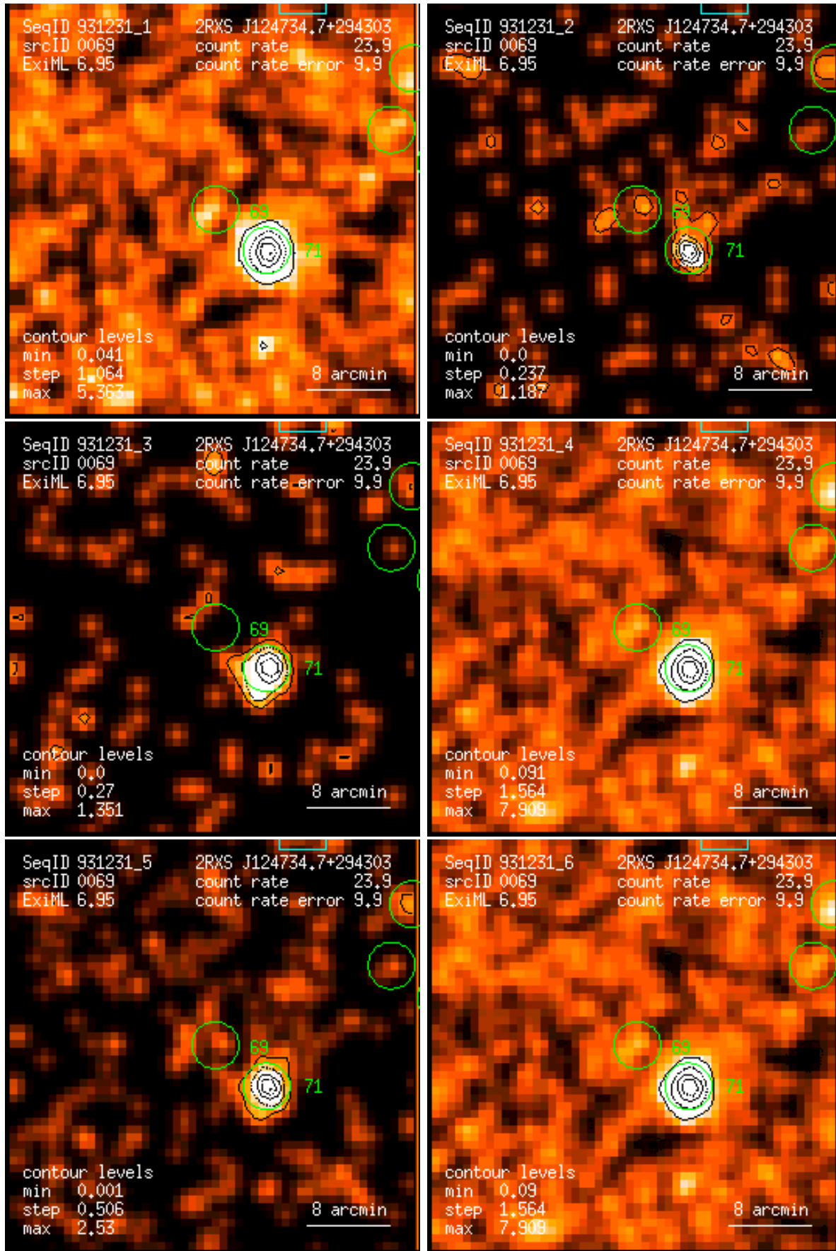
Figure 69: RASS 931231: detection 0069: band rate images, Gaussian filter: (1) PSPC channels 11 – 41, (2) 52 – 90, (3) 91 – 201, (4) 11 – 235, (5) 52 – 201, (6) 11 – 201. Broad band rates in counts/ks. Band rate contour levels in counts/ks/arcmin 2 .
