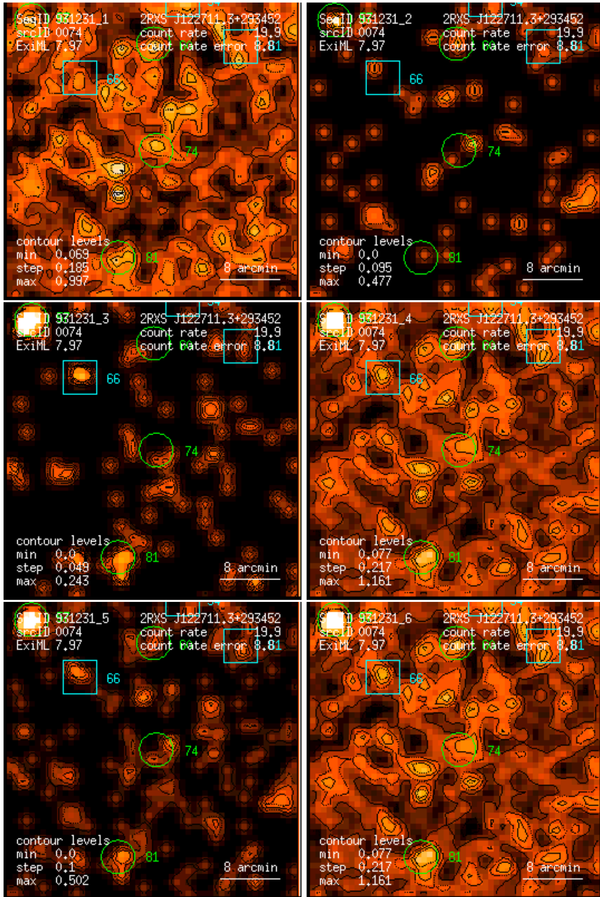
Figure 74: RASS 931231: detection 0074: band rate images, Gaussian filter: (1) PSPC channels 11 – 41, (2) 52 – 90, (3) 91 – 201, (4) 11 – 235, (5) 52 – 201, (6) 11 – 201. Broad band rates in counts/ks. Band rate contour levels in counts/ks/arcmin 2 .
