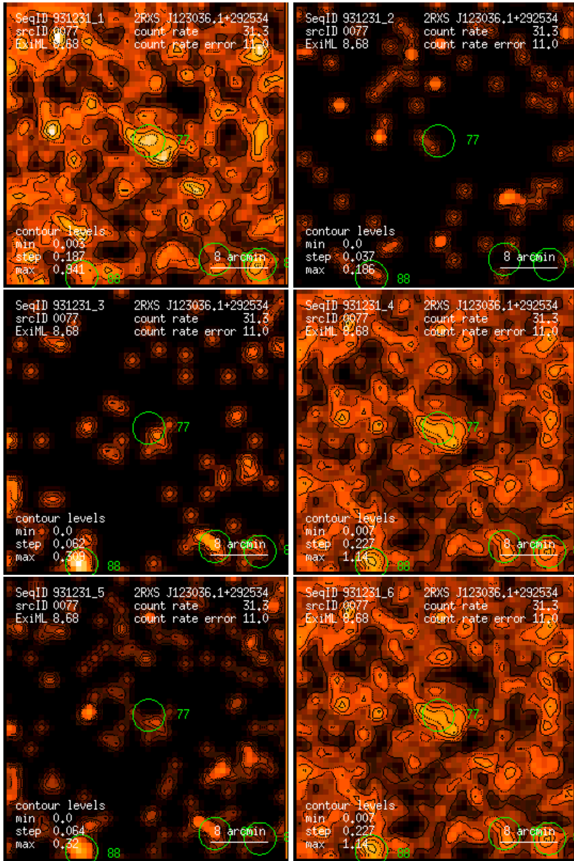
Figure 77: RASS 931231: detection 0077: band rate images, Gaussian filter: (1) PSPC channels 11 – 41, (2) 52 – 90, (3) 91 – 201, (4) 11 – 235, (5) 52 – 201, (6) 11 – 201. Broad band rates in counts/ks. Band rate contour levels in counts/ks/arcmin 2 .
