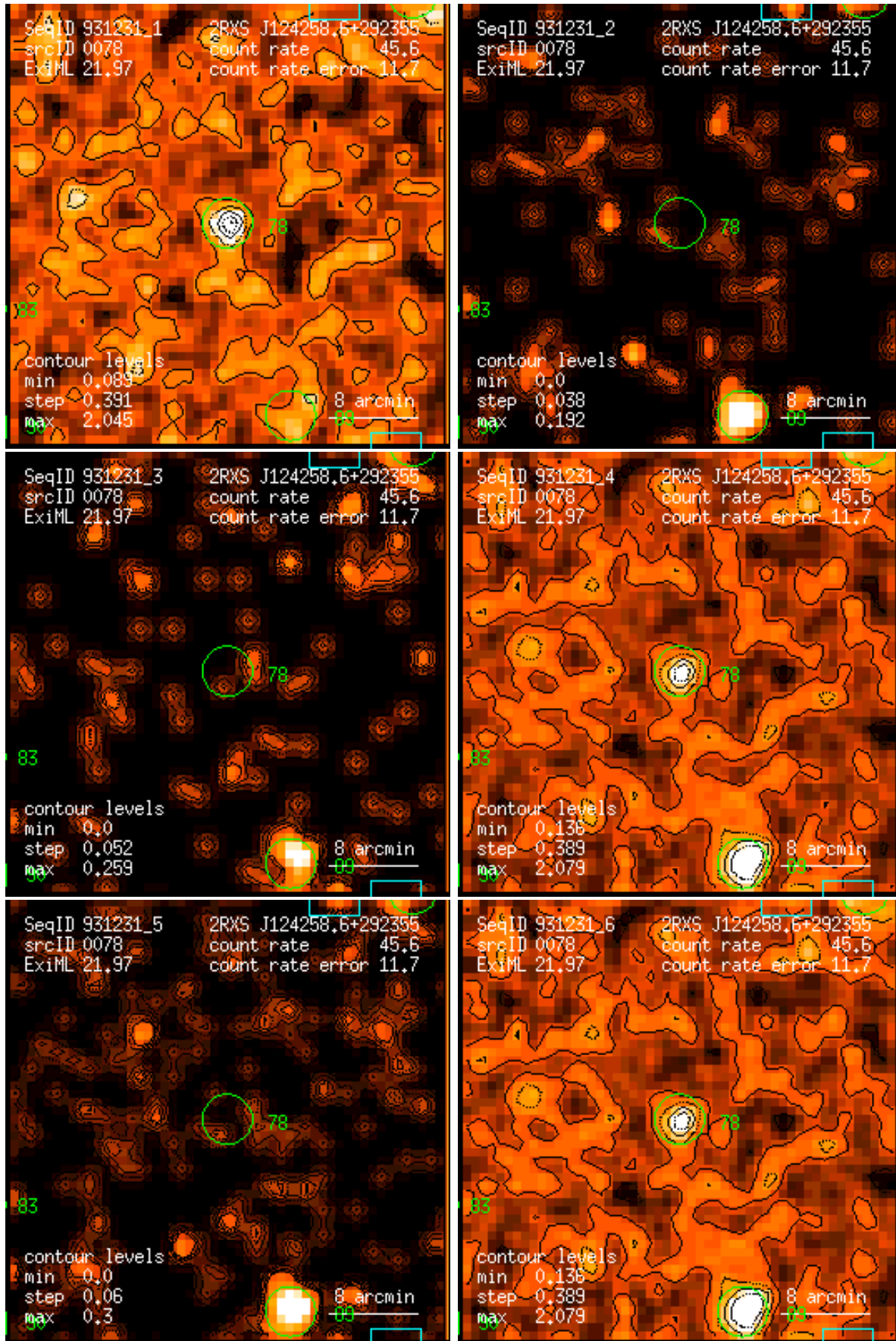
Figure 78: RASS 931231: detection 0078: band rate images, Gaussian filter: (1) PSPC channels 11 – 41, (2) 52 – 90, (3) 91 – 201, (4) 11 – 235, (5) 52 – 201, (6) 11 – 201. Broad band rates in counts/ks. Band rate contour levels in counts/ks/arcmin 2 .
