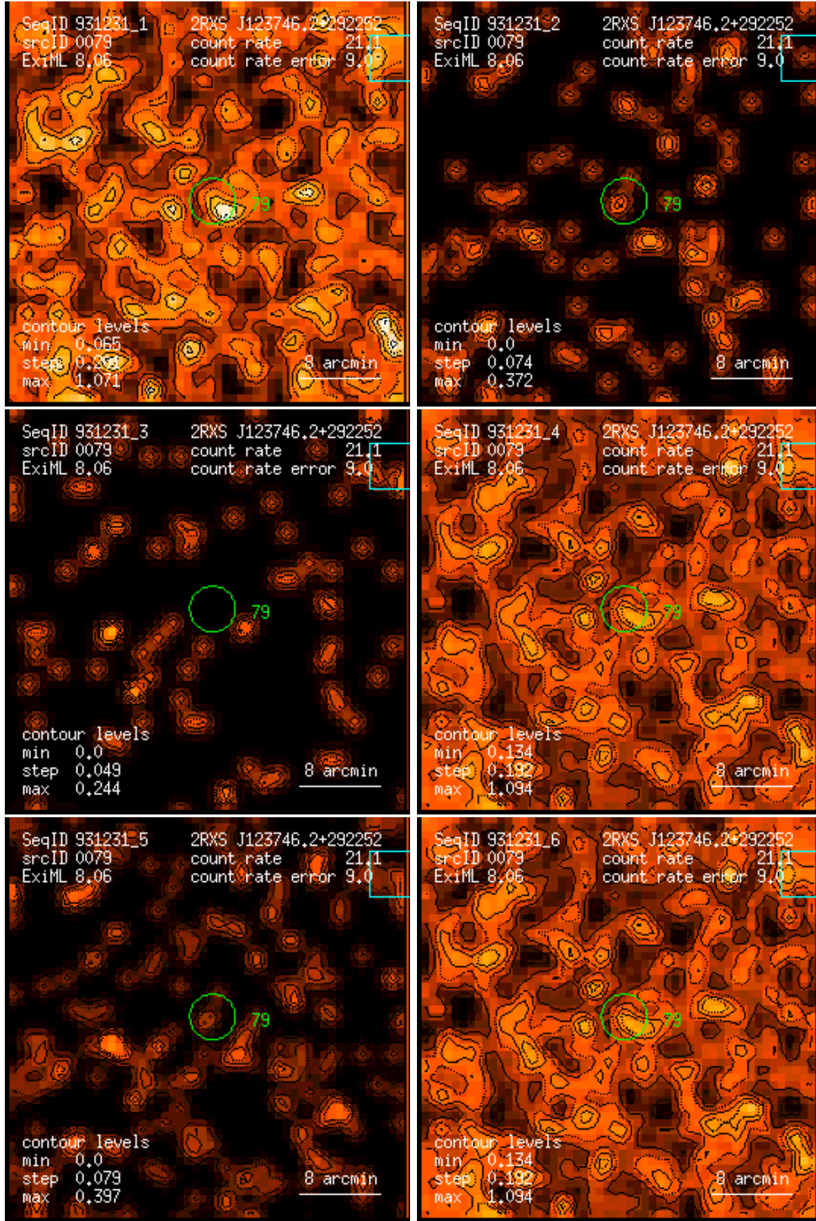
Figure 79: RASS 931231: detection 0079: band rate images, Gaussian filter: (1) PSPC channels 11 – 41, (2) 52 – 90, (3) 91 – 201, (4) 11 – 235, (5) 52 – 201, (6) 11 – 201. Broad band rates in counts/ks. Band rate contour levels in counts/ks/arcmin 2 .
