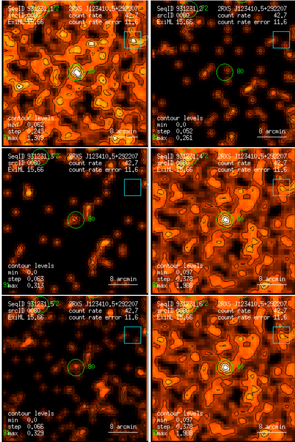
Figure 80: RASS 931231: detection 0080: band rate images, Gaussian filter: (1) PSPC channels 11 – 41, (2) 52 – 90, (3) 91 – 201, (4) 11 – 235, (5) 52 – 201, (6) 11 – 201. Broad band rates in counts/ks. Band rate contour levels in counts/ks/arcmin 2 .
