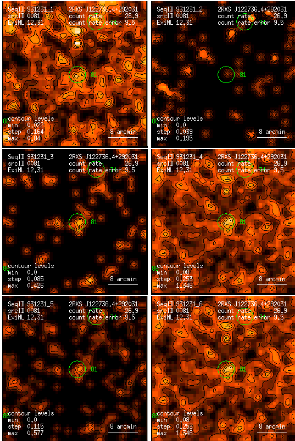
Figure 81: RASS 931231: detection 0081: band rate images, Gaussian filter: (1) PSPC channels 11 – 41, (2) 52 – 90, (3) 91 – 201, (4) 11 – 235, (5) 52 – 201, (6) 11 – 201. Broad band rates in counts/ks. Band rate contour levels in counts/ks/arcmin 2 .
