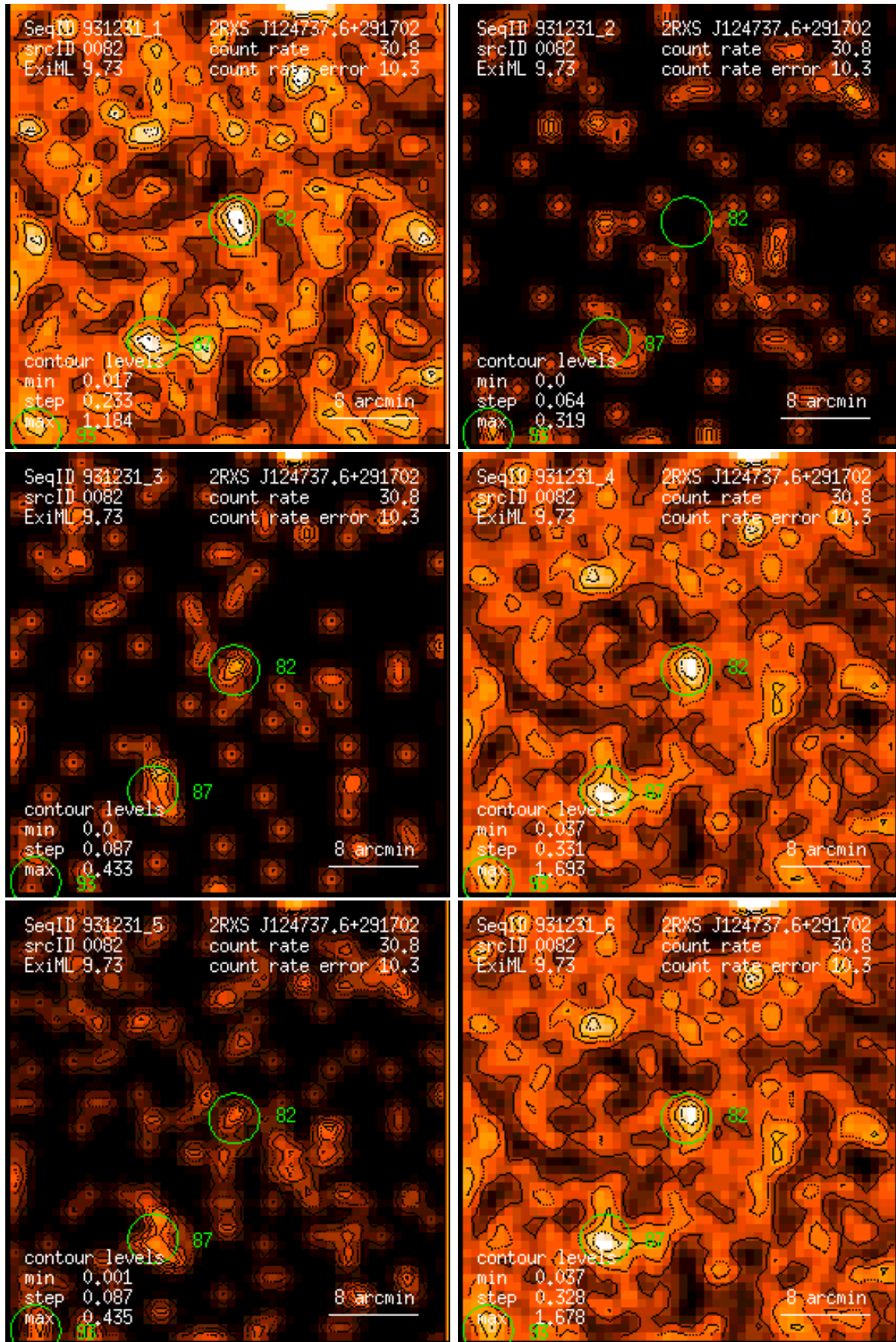
Figure 82: RASS 931231: detection 0082: band rate images, Gaussian filter: (1) PSPC channels 11 – 41, (2) 52 – 90, (3) 91 – 201, (4) 11 – 235, (5) 52 – 201, (6) 11 – 201. Broad band rates in counts/ks. Band rate contour levels in counts/ks/arcmin 2 .
