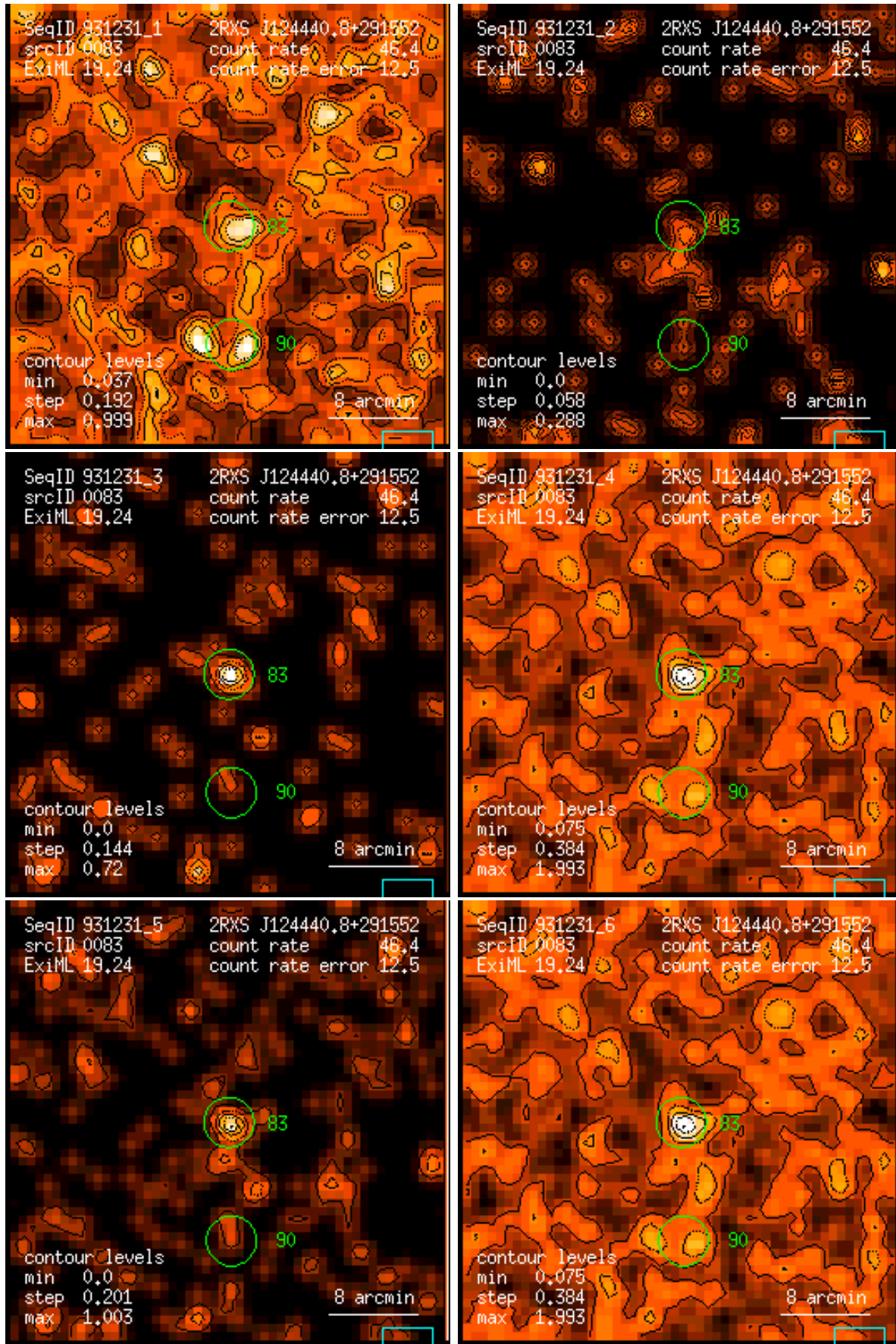
Figure 83: RASS 931231: detection 0083: band rate images, Gaussian filter: (1) PSPC channels 11 – 41, (2) 52 – 90, (3) 91 – 201, (4) 11 – 235, (5) 52 – 201, (6) 11 – 201. Broad band rates in counts/ks. Band rate contour levels in counts/ks/arcmin 2 .
