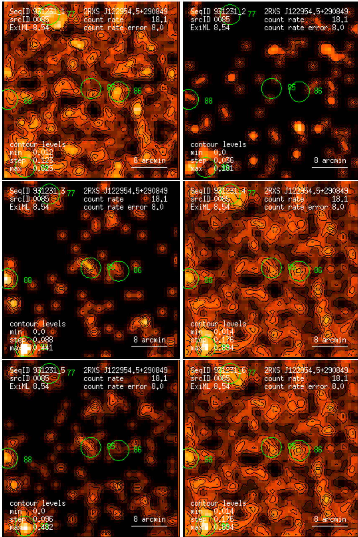
Figure 85: RASS 931231: detection 0085: band rate images, Gaussian filter: (1) PSPC channels 11 – 41, (2) 52 – 90, (3) 91 – 201, (4) 11 – 235, (5) 52 – 201, (6) 11 – 201. Broad band rates in counts/ks. Band rate contour levels in counts/ks/arcmin 2 .
